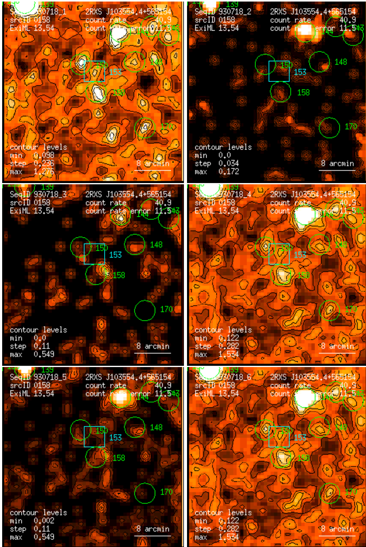
Figure 158: RASS 930718: detection 0158: band rate images, Gaussian filter: (1) PSPC channels 11 – 41, (2) 52 – 90, (3) 91 – 201, (4) 11 – 235, (5) 52 – 201, (6) 11 – 201. Broad band rates in counts/ks. Band rate contour levels in counts/ks/arcmin 2 .
