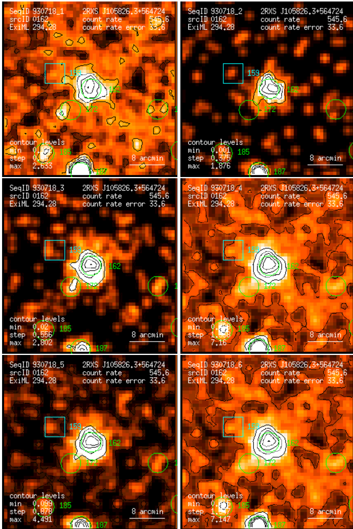
Figure 162: RASS 930718: detection 0162: band rate images, Gaussian filter: (1) PSPC channels 11 – 41, (2) 52 – 90, (3) 91 – 201, (4) 11 – 235, (5) 52 – 201, (6) 11 – 201. Broad band rates in counts/ks. Band rate contour levels in counts/ks/arcmin 2 .
