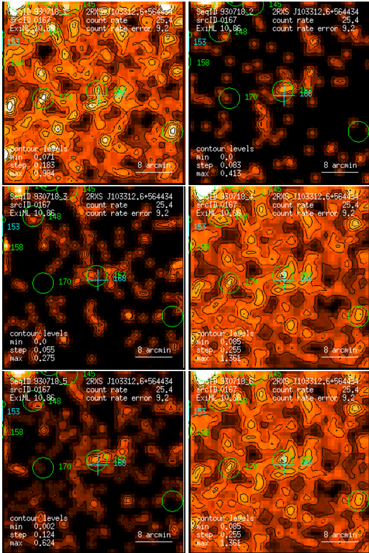
Figure 167: RASS 930718: detection 0167: band rate images, Gaussian filter: (1) PSPC channels 11 – 41, (2) 52 – 90, (3) 91 – 201, (4) 11 – 235, (5) 52 – 201, (6) 11 – 201. Broad band rates in counts/ks. Band rate contour levels in counts/ks/arcmin 2 .
