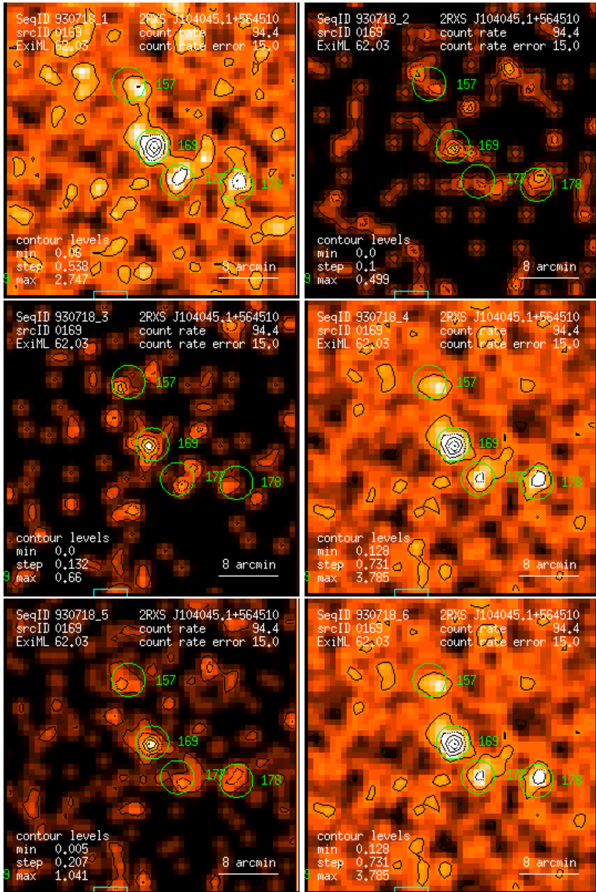
Figure 169: RASS 930718: detection 0169: band rate images, Gaussian filter: (1) PSPC channels 11 – 41, (2) 52 – 90, (3) 91 – 201, (4) 11 – 235, (5) 52 – 201, (6) 11 – 201. Broad band rates in counts/ks. Band rate contour levels in counts/ks/arcmin 2 .
