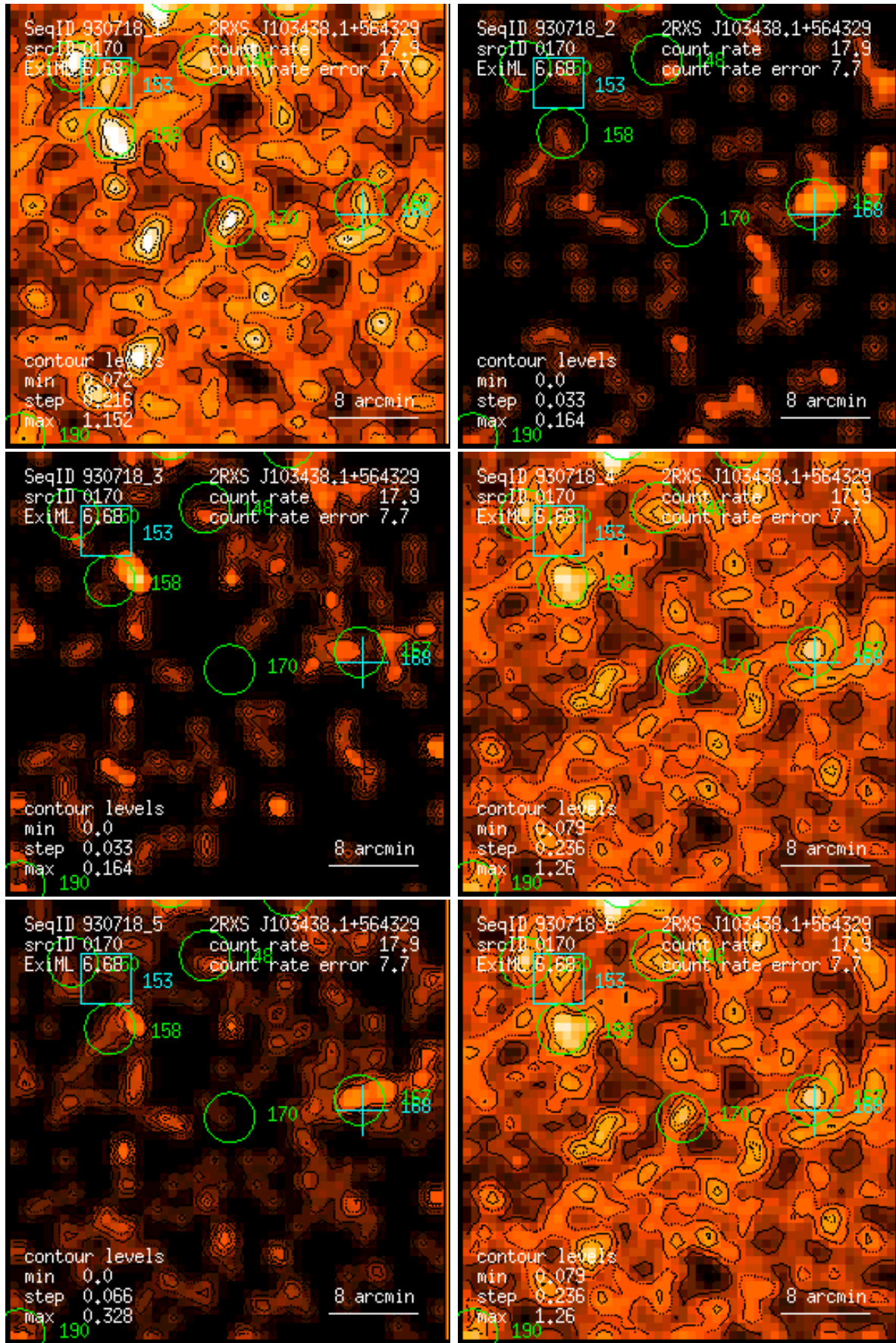
Figure 170: RASS 930718: detection 0170: band rate images, Gaussian filter: (1) PSPC channels 11 – 41, (2) 52 – 90, (3) 91 – 201, (4) 11 – 235, (5) 52 – 201, (6) 11 – 201. Broad band rates in counts/ks. Band rate contour levels in counts/ks/arcmin 2 .
