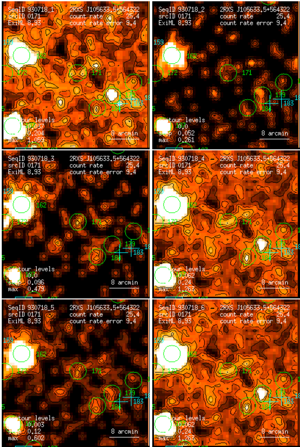
Figure 171: RASS 930718: detection 0171: band rate images, Gaussian filter: (1) PSPC channels 11 – 41, (2) 52 – 90, (3) 91 – 201, (4) 11 – 235, (5) 52 – 201, (6) 11 – 201. Broad band rates in counts/ks. Band rate contour levels in counts/ks/arcmin 2 .
