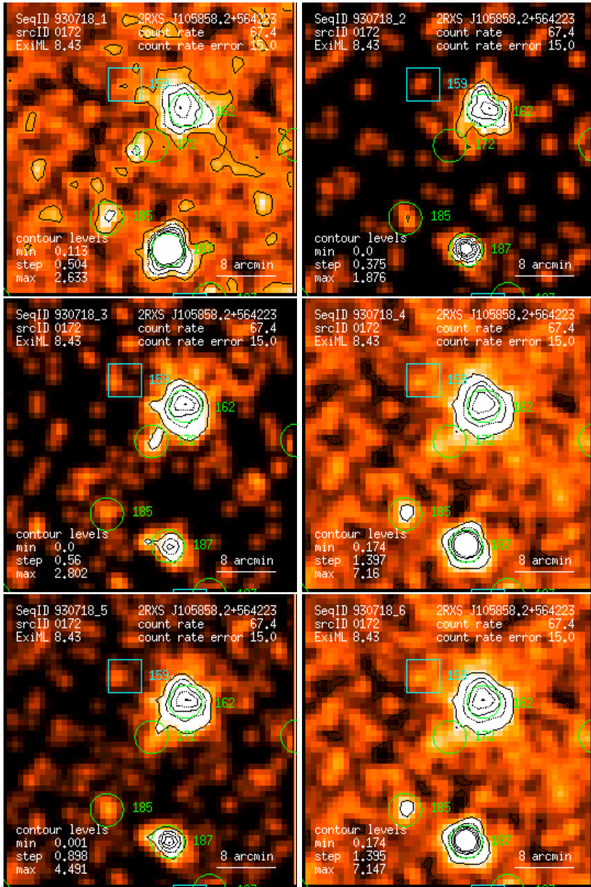
Figure 172: RASS 930718: detection 0172: band rate images, Gaussian filter: (1) PSPC channels 11 – 41, (2) 52 – 90, (3) 91 – 201, (4) 11 – 235, (5) 52 – 201, (6) 11 – 201. Broad band rates in counts/ks. Band rate contour levels in counts/ks/arcmin 2 .
