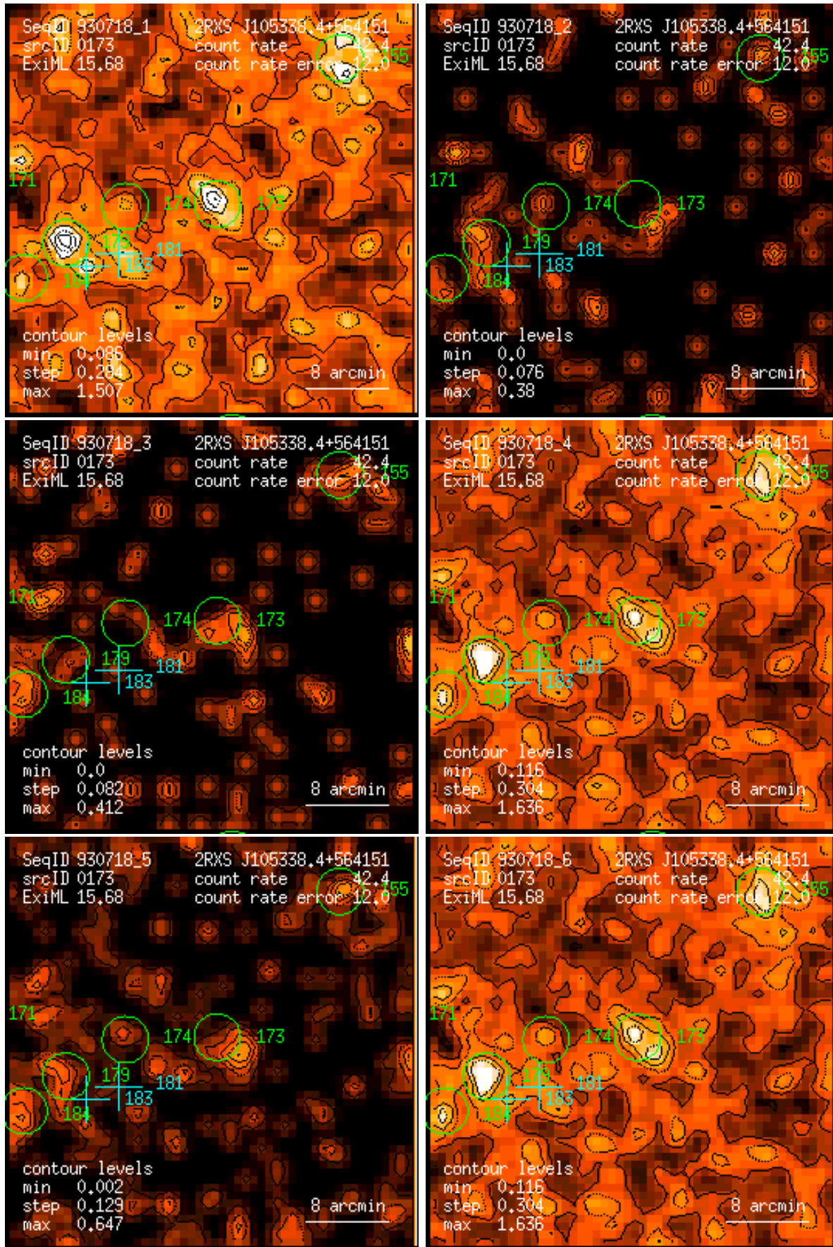
Figure 173: RASS 930718: detection 0173: band rate images, Gaussian filter: (1) PSPC channels 11 – 41, (2) 52 – 90, (3) 91 – 201, (4) 11 – 235, (5) 52 – 201, (6) 11 – 201. Broad band rates in counts/ks. Band rate contour levels in counts/ks/arcmin 2 .
