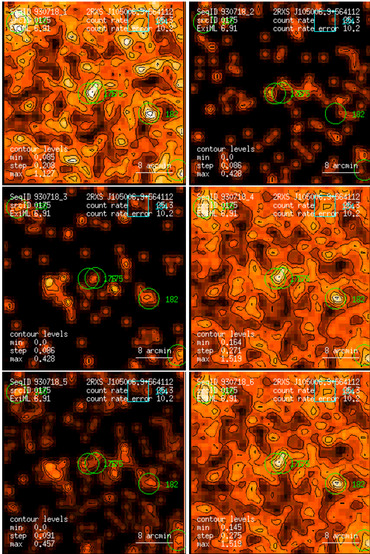
Figure 175: RASS 930718: detection 0175: band rate images, Gaussian filter: (1) PSPC channels 11 – 41, (2) 52 – 90, (3) 91 – 201, (4) 11 – 235, (5) 52 – 201, (6) 11 – 201. Broad band rates in counts/ks. Band rate contour levels in counts/ks/arcmin 2 .
