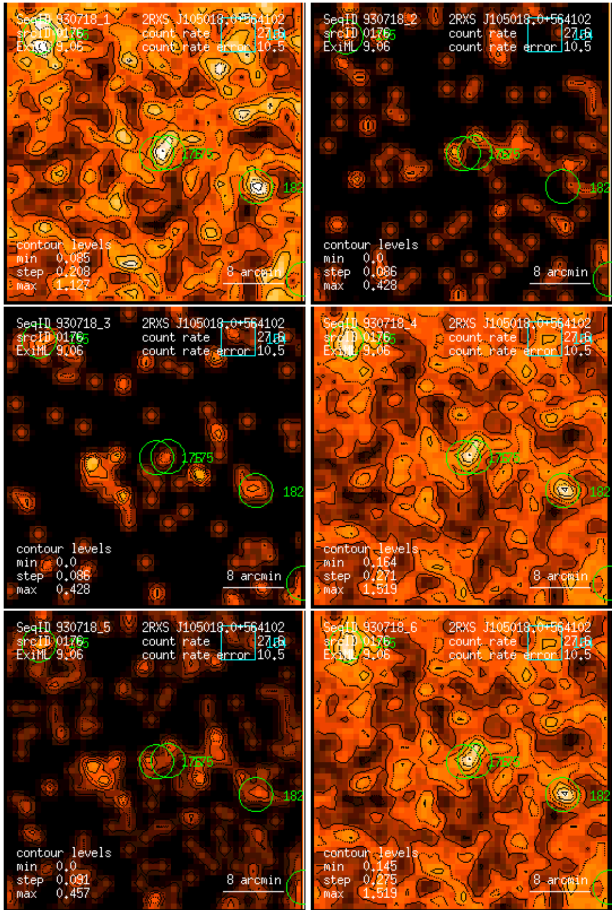
Figure 176: RASS 930718: detection 0176: band rate images, Gaussian filter: (1) PSPC channels 11 – 41, (2) 52 – 90, (3) 91 – 201, (4) 11 – 235, (5) 52 – 201, (6) 11 – 201. Broad band rates in counts/ks. Band rate contour levels in counts/ks/arcmin 2 .
