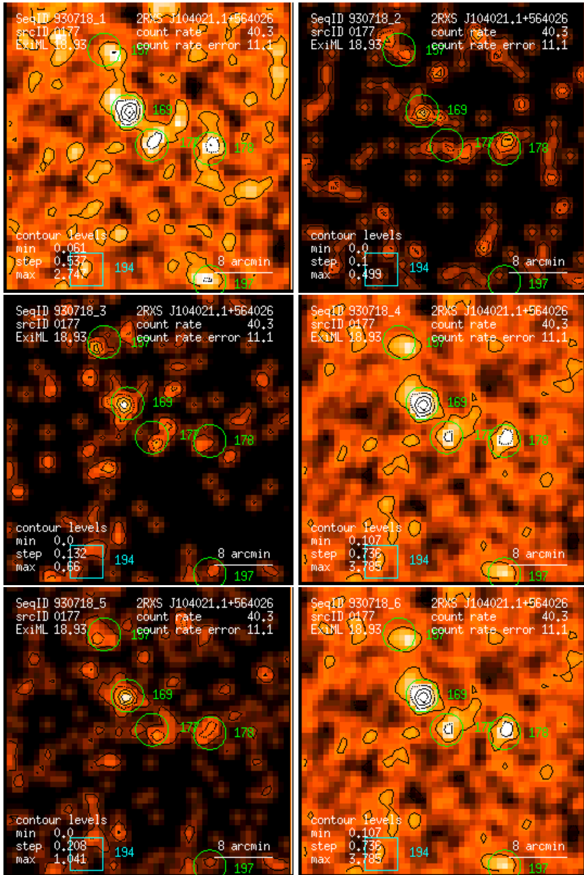
Figure 177: RASS 930718: detection 0177: band rate images, Gaussian filter: (1) PSPC channels 11 – 41, (2) 52 – 90, (3) 91 – 201, (4) 11 – 235, (5) 52 – 201, (6) 11 – 201. Broad band rates in counts/ks. Band rate contour levels in counts/ks/arcmin 2 .
