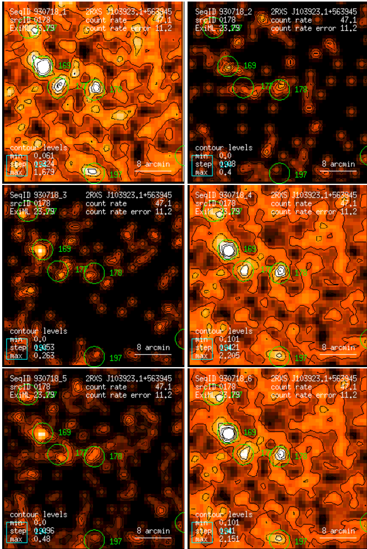
Figure 178: RASS 930718: detection 0178: band rate images, Gaussian filter: (1) PSPC channels 11 – 41, (2) 52 – 90, (3) 91 – 201, (4) 11 – 235, (5) 52 – 201, (6) 11 – 201. Broad band rates in counts/ks. Band rate contour levels in counts/ks/arcmin 2 .
