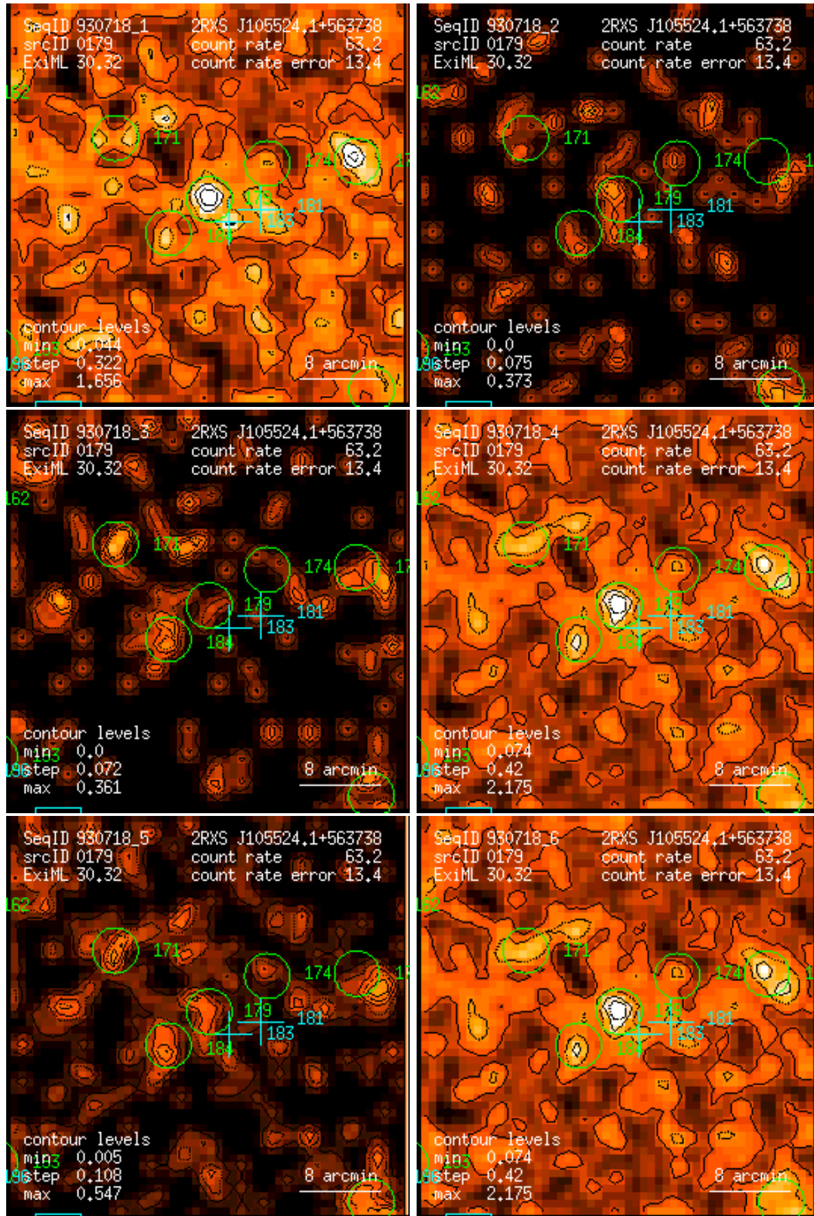
Figure 179: RASS 930718: detection 0179: band rate images, Gaussian filter: (1) PSPC channels 11 – 41, (2) 52 – 90, (3) 91 – 201, (4) 11 – 235, (5) 52 – 201, (6) 11 – 201. Broad band rates in counts/ks. Band rate contour levels in counts/ks/arcmin 2 .
