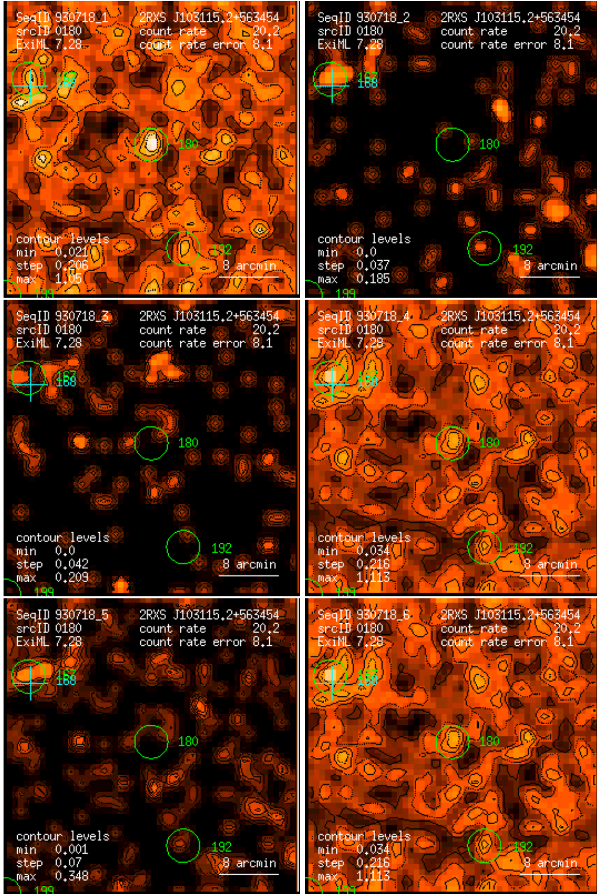
Figure 180: RASS 930718: detection 0180: band rate images, Gaussian filter: (1) PSPC channels 11 – 41, (2) 52 – 90, (3) 91 – 201, (4) 11 – 235, (5) 52 – 201, (6) 11 – 201. Broad band rates in counts/ks. Band rate contour levels in counts/ks/arcmin 2 .
