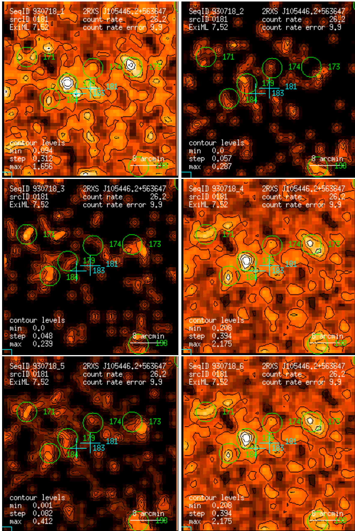
Figure 181: RASS 930718: detection 0181: band rate images, Gaussian filter: (1) PSPC channels 11 – 41, (2) 52 – 90, (3) 91 – 201, (4) 11 – 235, (5) 52 – 201, (6) 11 – 201. Broad band rates in counts/ks. Band rate contour levels in counts/ks/arcmin 2 .
