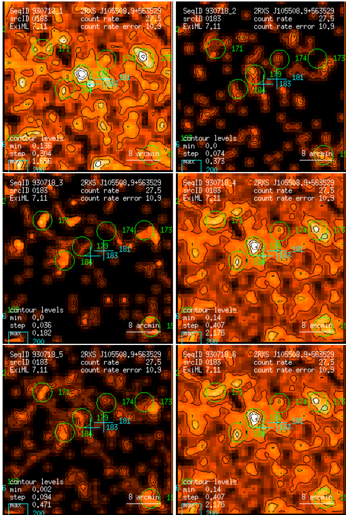
Figure 183: RASS 930718: detection 0183: band rate images, Gaussian filter: (1) PSPC channels 11 – 41, (2) 52 – 90, (3) 91 – 201, (4) 11 – 235, (5) 52 – 201, (6) 11 – 201. Broad band rates in counts/ks. Band rate contour levels in counts/ks/arcmin 2 .
