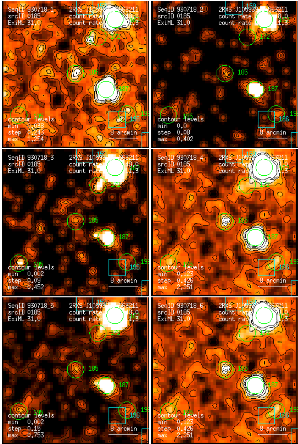
Figure 185: RASS 930718: detection 0185: band rate images, Gaussian filter: (1) PSPC channels 11 – 41, (2) 52 – 90, (3) 91 – 201, (4) 11 – 235, (5) 52 – 201, (6) 11 – 201. Broad band rates in counts/ks. Band rate contour levels in counts/ks/arcmin 2 .
