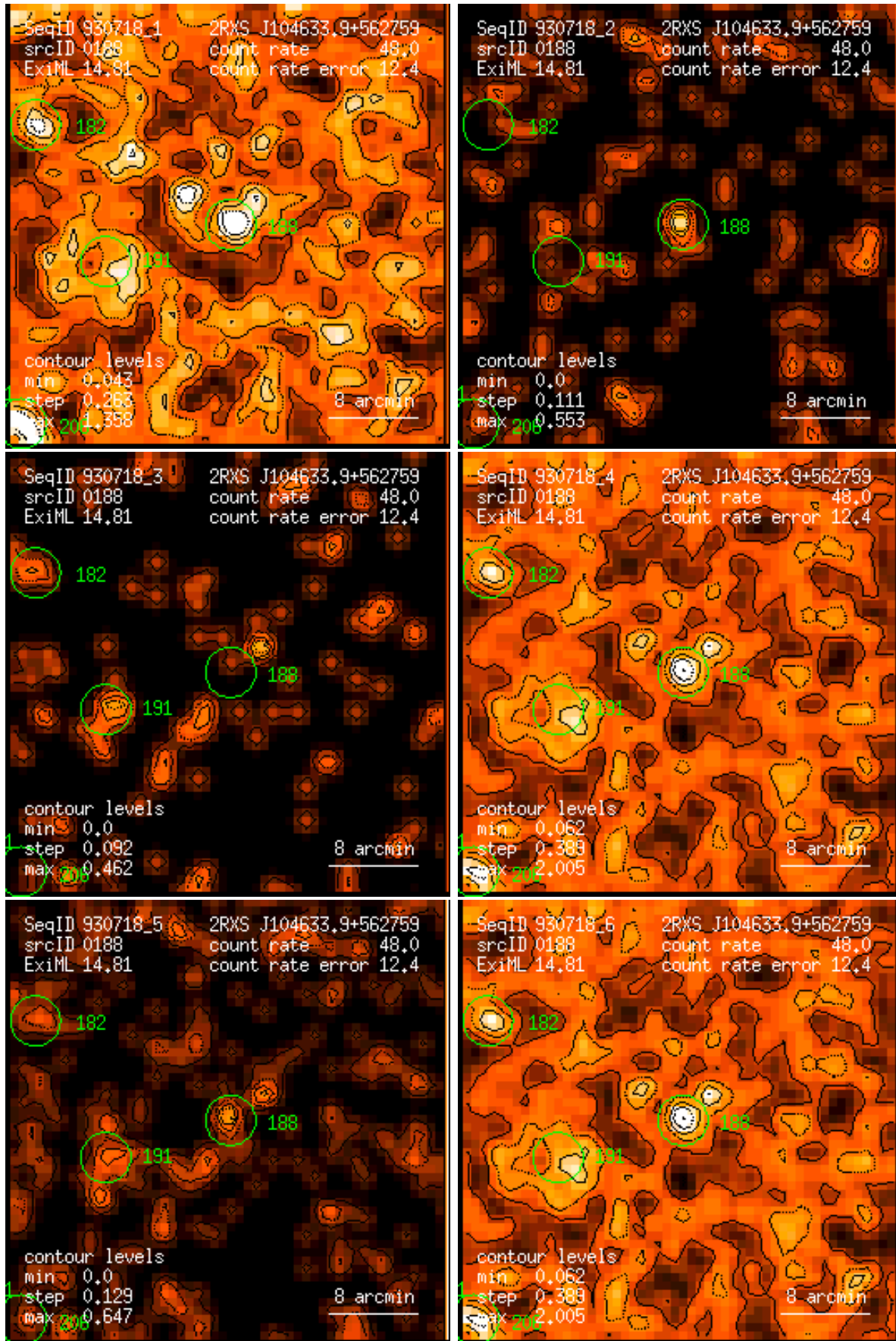
Figure 188: RASS 930718: detection 0188: band rate images, Gaussian filter: (1) PSPC channels 11 – 41, (2) 52 – 90, (3) 91 – 201, (4) 11 – 235, (5) 52 – 201, (6) 11 – 201. Broad band rates in counts/ks. Band rate contour levels in counts/ks/arcmin 2 .
