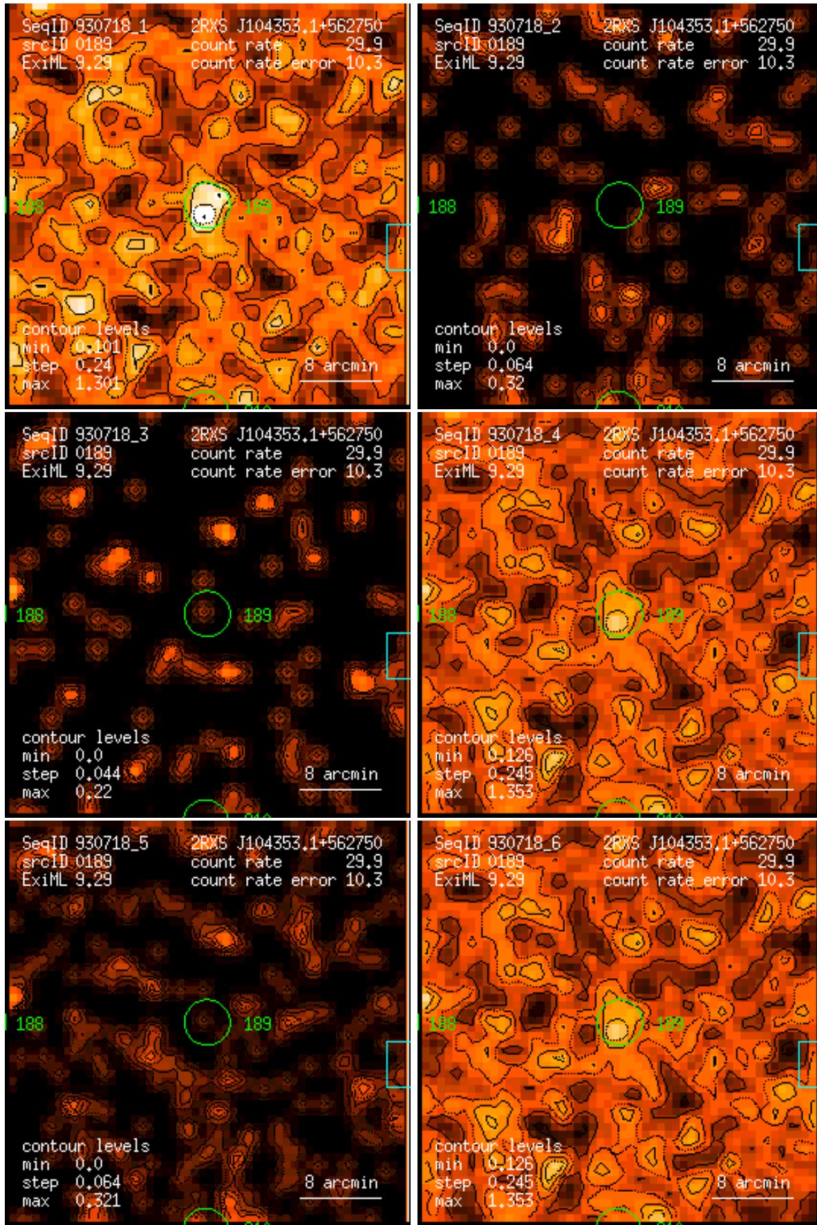
Figure 189: RASS 930718: detection 0189: band rate images, Gaussian filter: (1) PSPC channels 11 – 41, (2) 52 – 90, (3) 91 – 201, (4) 11 – 235, (5) 52 – 201, (6) 11 – 201. Broad band rates in counts/ks. Band rate contour levels in counts/ks/arcmin 2 .
