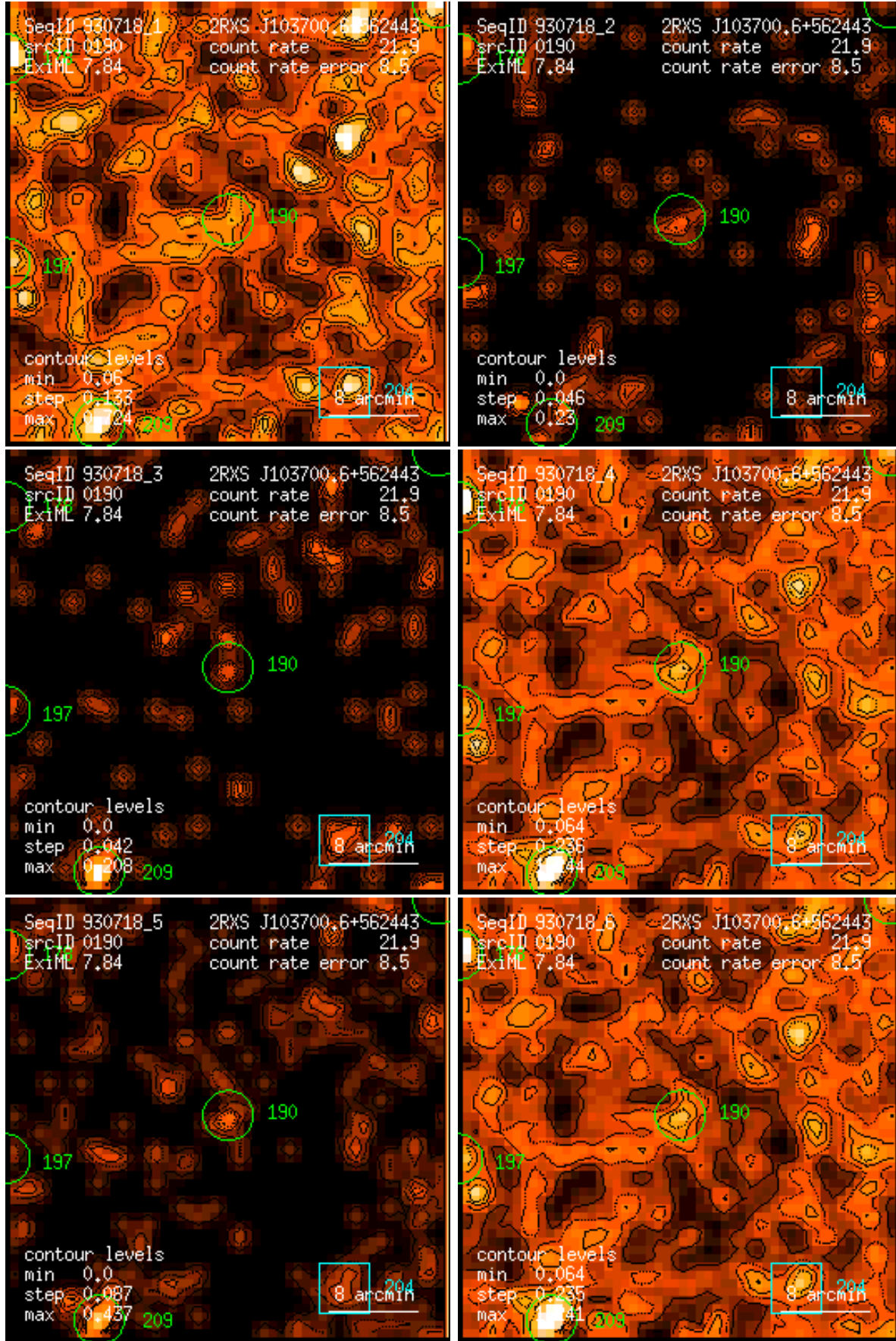
Figure 190: RASS 930718: detection 0190: band rate images, Gaussian filter: (1) PSPC channels 11 – 41, (2) 52 – 90, (3) 91 – 201, (4) 11 – 235, (5) 52 – 201, (6) 11 – 201. Broad band rates in counts/ks. Band rate contour levels in counts/ks/arcmin 2 .
