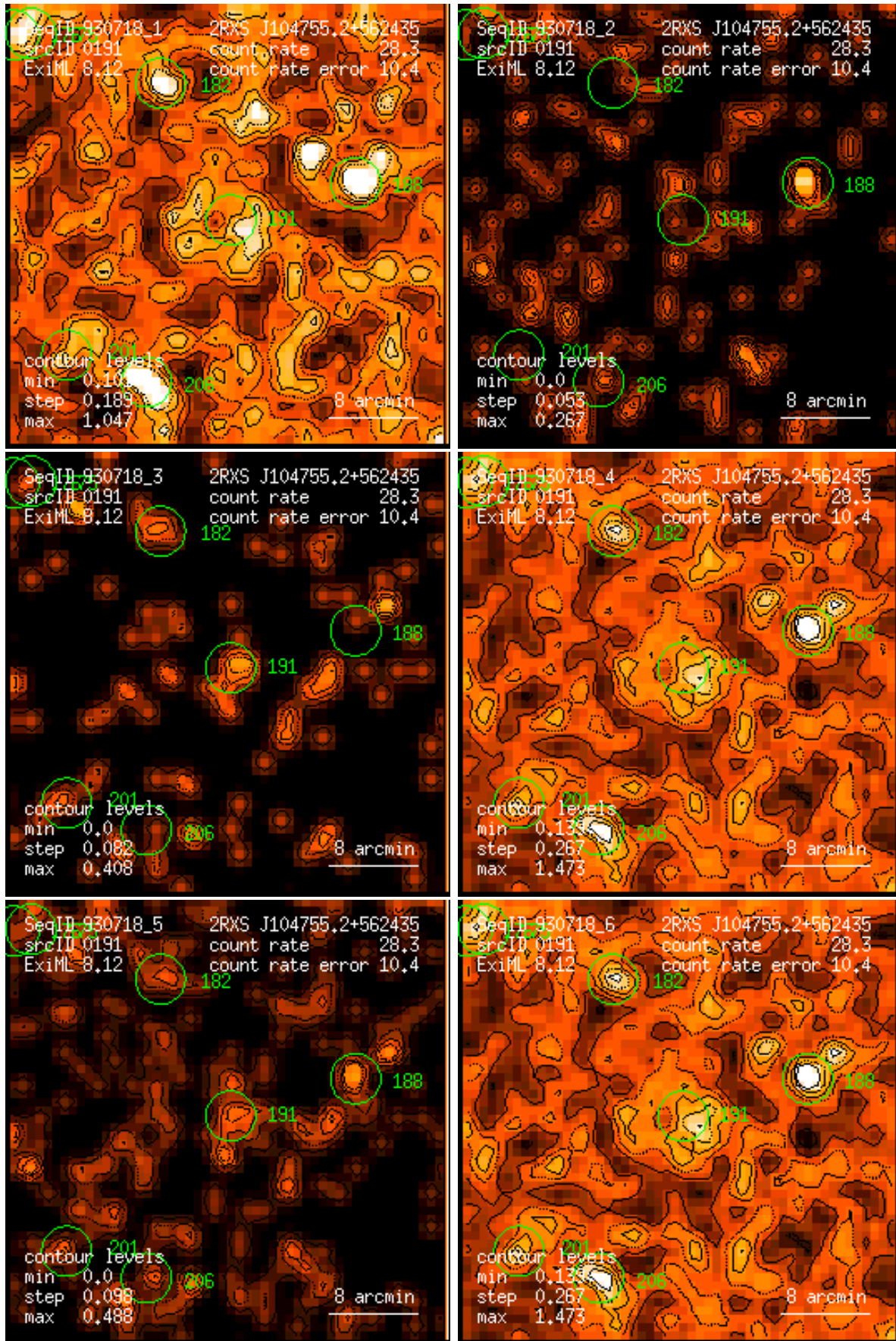
Figure 191: RASS 930718: detection 0191: band rate images, Gaussian filter: (1) PSPC channels 11 – 41, (2) 52 – 90, (3) 91 – 201, (4) 11 – 235, (5) 52 – 201, (6) 11 – 201. Broad band rates in counts/ks. Band rate contour levels in counts/ks/arcmin 2 .
