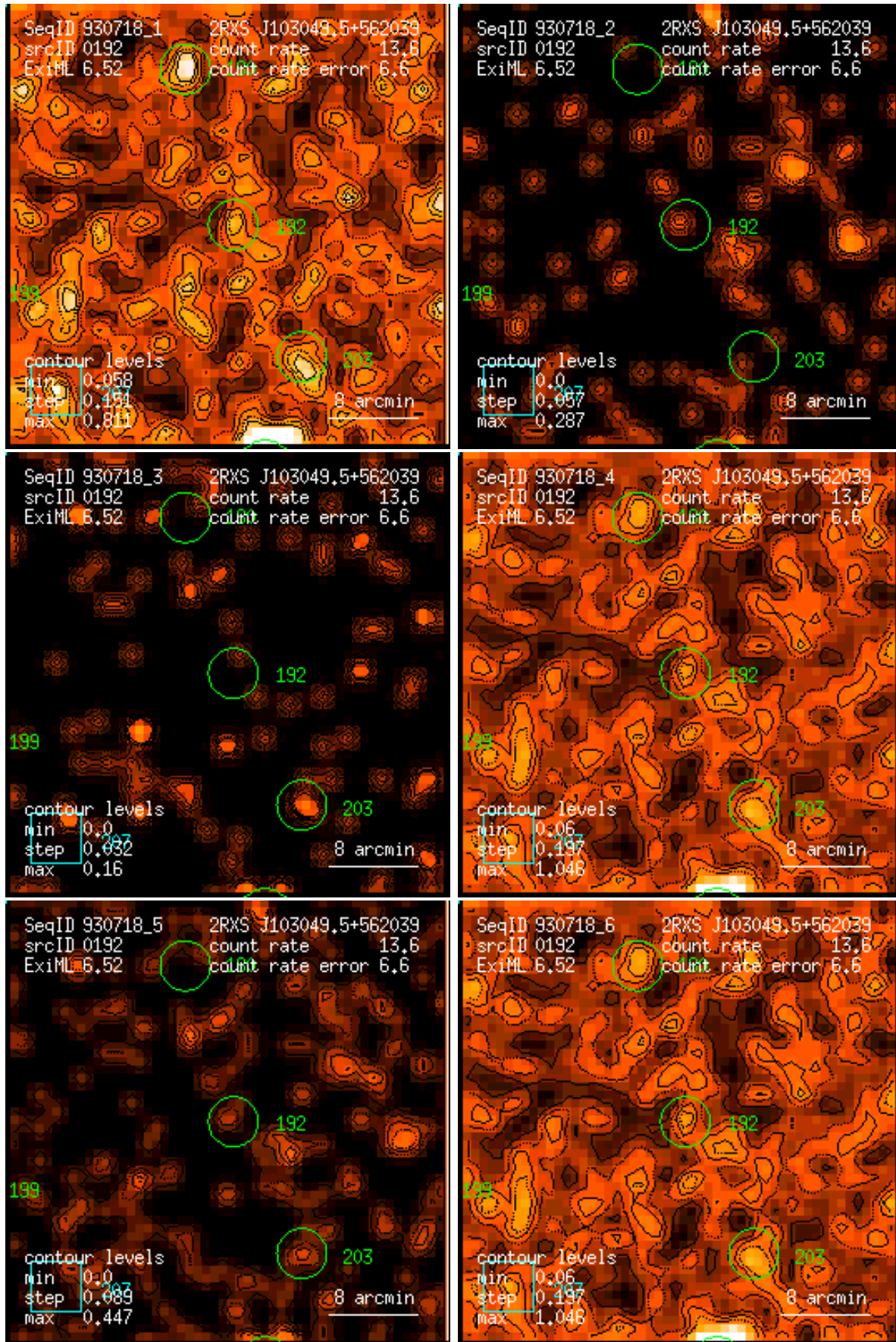
Figure 192: RASS 930718: detection 0192: band rate images, Gaussian filter: (1) PSPC channels 11 – 41, (2) 52 – 90, (3) 91 – 201, (4) 11 – 235, (5) 52 – 201, (6) 11 – 201. Broad band rates in counts/ks. Band rate contour levels in counts/ks/arcmin 2 .
