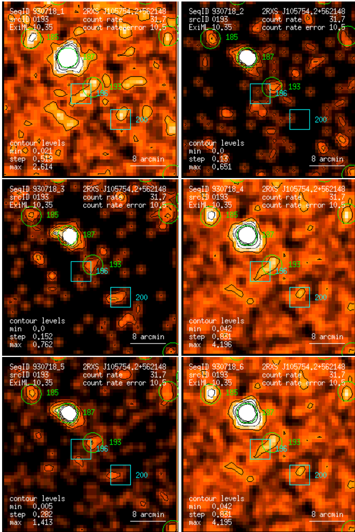
Figure 193: RASS 930718: detection 0193: band rate images, Gaussian filter: (1) PSPC channels 11 – 41, (2) 52 – 90, (3) 91 – 201, (4) 11 – 235, (5) 52 – 201, (6) 11 – 201. Broad band rates in counts/ks. Band rate contour levels in counts/ks/arcmin 2 .
