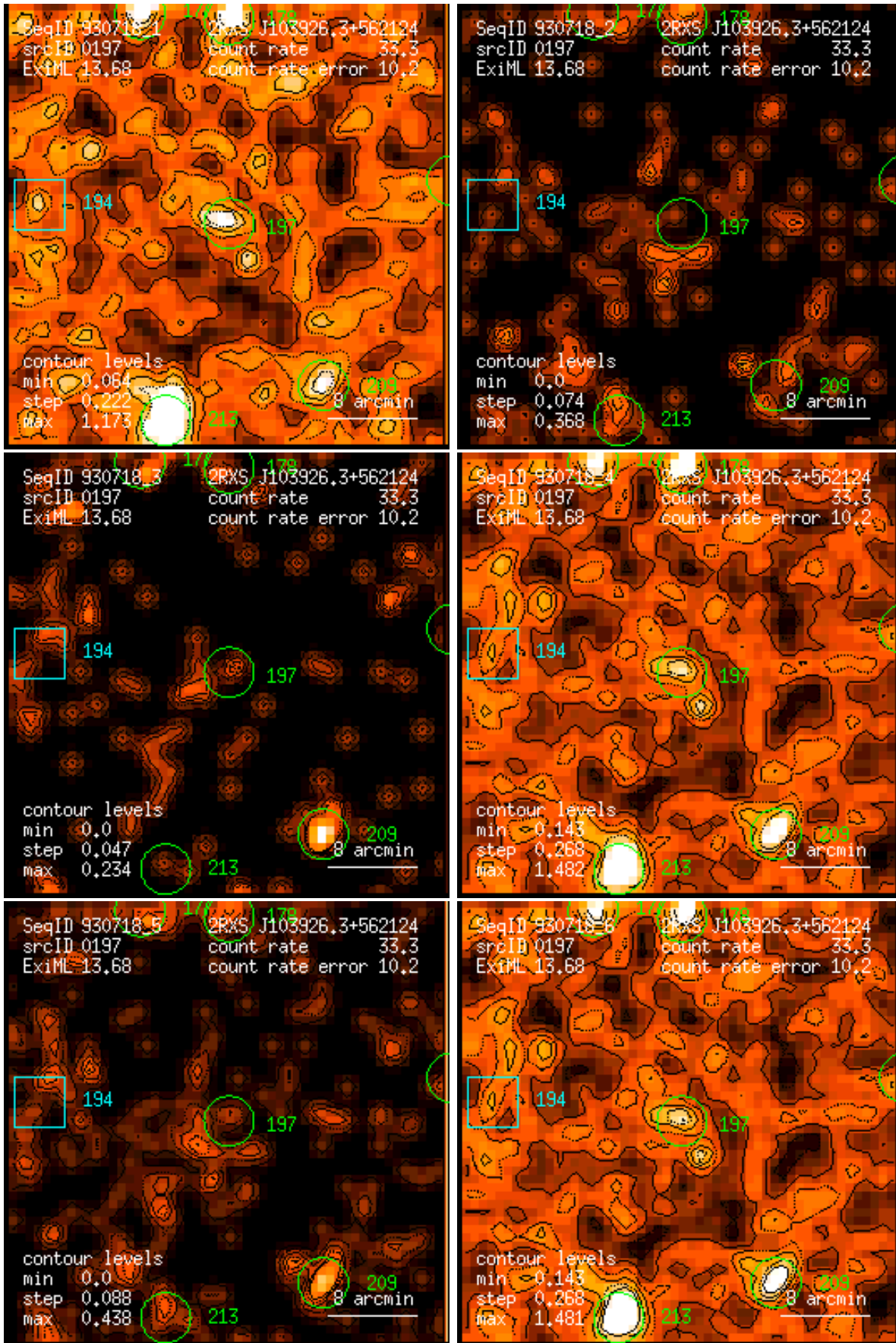
Figure 197: RASS 930718: detection 0197: band rate images, Gaussian filter: (1) PSPC channels 11 – 41, (2) 52 – 90, (3) 91 – 201, (4) 11 – 235, (5) 52 – 201, (6) 11 – 201. Broad band rates in counts/ks. Band rate contour levels in counts/ks/arcmin 2 .
