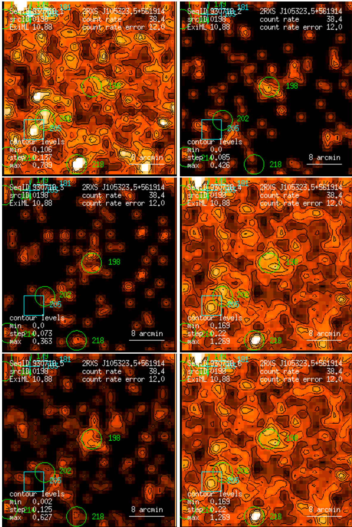
Figure 198: RASS 930718: detection 0198: band rate images, Gaussian filter: (1) PSPC channels 11 – 41, (2) 52 – 90, (3) 91 – 201, (4) 11 – 235, (5) 52 – 201, (6) 11 – 201. Broad band rates in counts/ks. Band rate contour levels in counts/ks/arcmin 2 .
