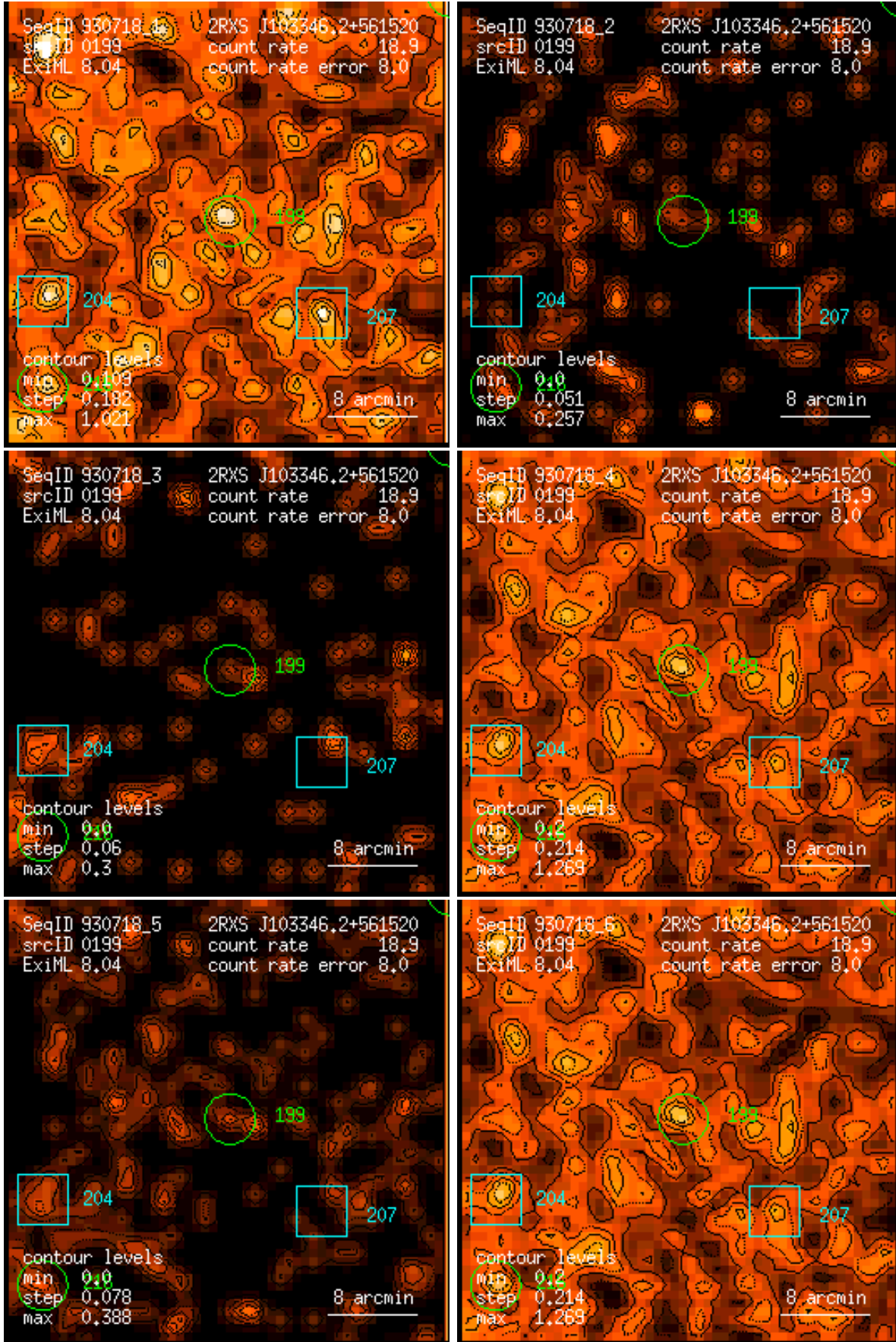
Figure 199: RASS 930718: detection 0199: band rate images, Gaussian filter: (1) PSPC channels 11 – 41, (2) 52 – 90, (3) 91 – 201, (4) 11 – 235, (5) 52 – 201, (6) 11 – 201. Broad band rates in counts/ks. Band rate contour levels in counts/ks/arcmin 2 .
