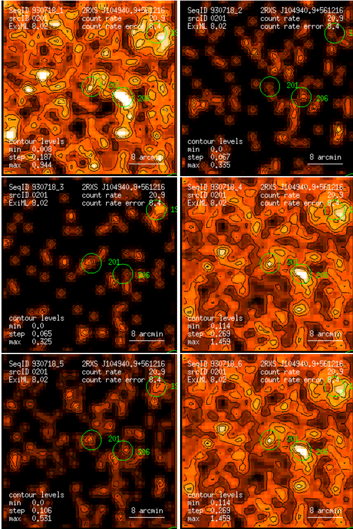
Figure 201: RASS 930718: detection 0201: band rate images, Gaussian filter: (1) PSPC channels 11 – 41, (2) 52 – 90, (3) 91 – 201, (4) 11 – 235, (5) 52 – 201, (6) 11 – 201. Broad band rates in counts/ks. Band rate contour levels in counts/ks/arcmin 2 .
