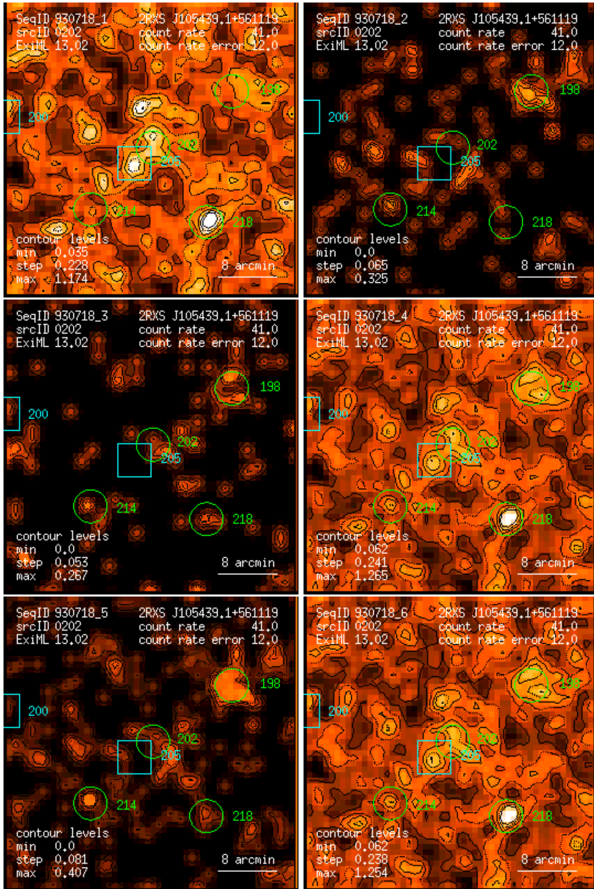
Figure 202: RASS 930718: detection 0202: band rate images, Gaussian filter: (1) PSPC channels 11 – 41, (2) 52 – 90, (3) 91 – 201, (4) 11 – 235, (5) 52 – 201, (6) 11 – 201. Broad band rates in counts/ks. Band rate contour levels in counts/ks/arcmin 2 .
