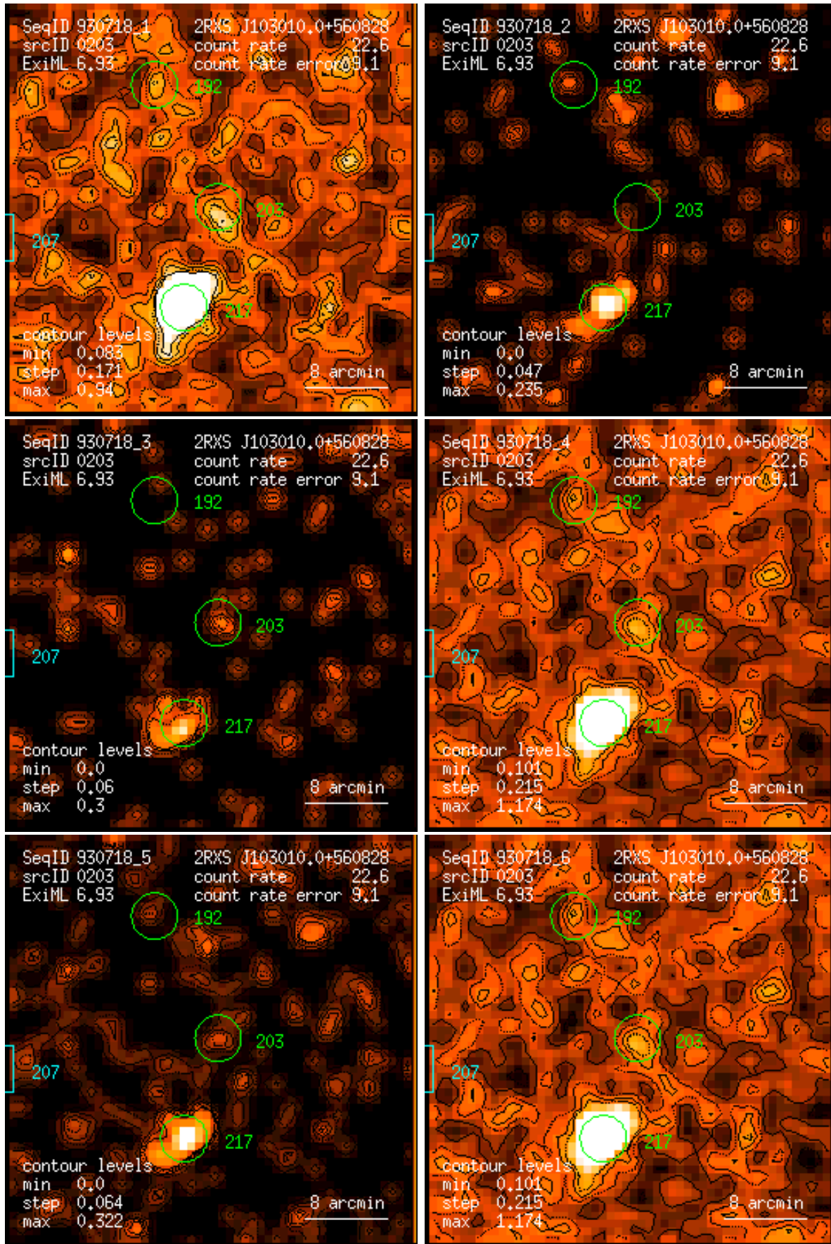
Figure 203: RASS 930718: detection 0203: band rate images, Gaussian filter: (1) PSPC channels 11 – 41, (2) 52 – 90, (3) 91 – 201, (4) 11 – 235, (5) 52 – 201, (6) 11 – 201. Broad band rates in counts/ks. Band rate contour levels in counts/ks/arcmin 2 .
