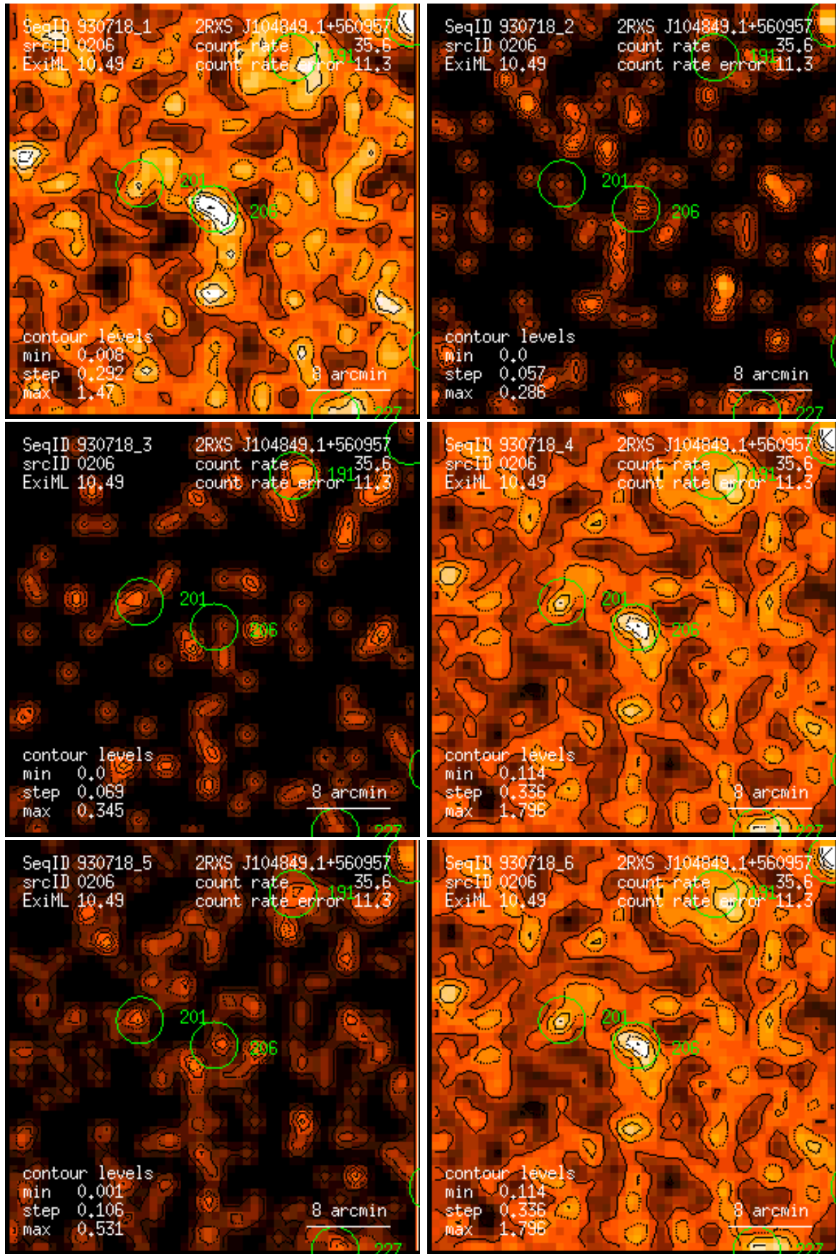
Figure 206: RASS 930718: detection 0206: band rate images, Gaussian filter: (1) PSPC channels 11 – 41, (2) 52 – 90, (3) 91 – 201, (4) 11 – 235, (5) 52 – 201, (6) 11 – 201. Broad band rates in counts/ks. Band rate contour levels in counts/ks/arcmin 2 .
