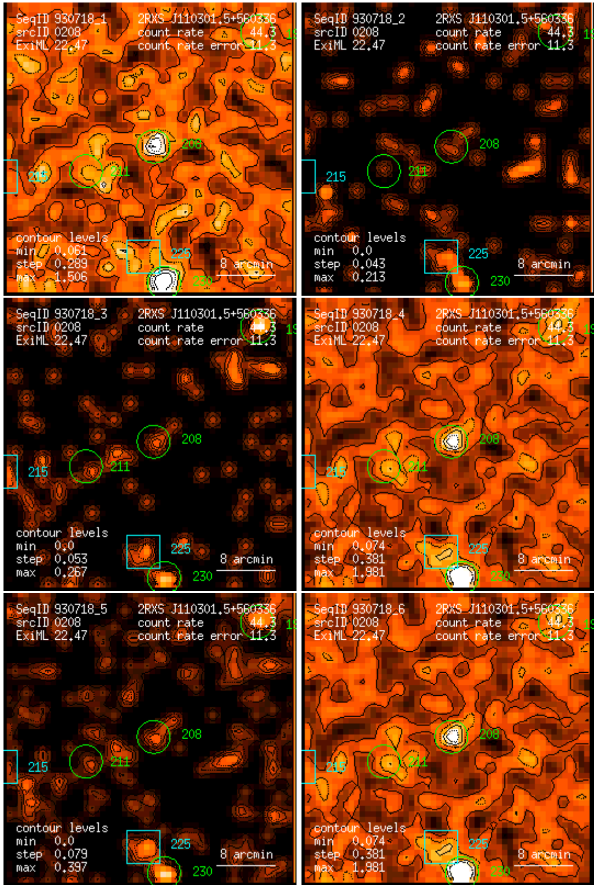
Figure 208: RASS 930718: detection 0208: band rate images, Gaussian filter: (1) PSPC channels 11 – 41, (2) 52 – 90, (3) 91 – 201, (4) 11 – 235, (5) 52 – 201, (6) 11 – 201. Broad band rates in counts/ks. Band rate contour levels in counts/ks/arcmin 2 .
