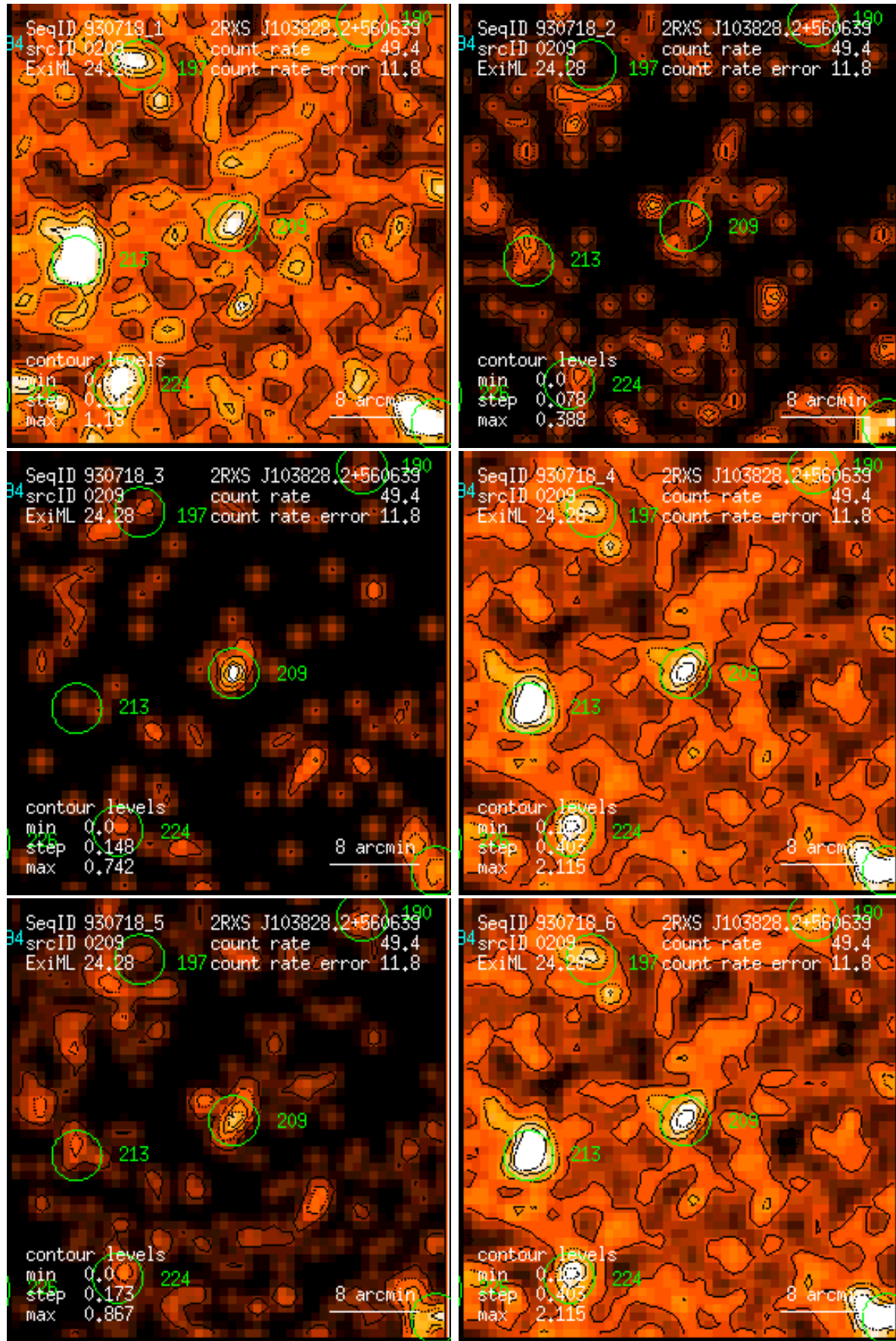
Figure 209: RASS 930718: detection 0209: band rate images, Gaussian filter: (1) PSPC channels 11 – 41, (2) 52 – 90, (3) 91 – 201, (4) 11 – 235, (5) 52 – 201, (6) 11 – 201. Broad band rates in counts/ks. Band rate contour levels in counts/ks/arcmin 2 .
