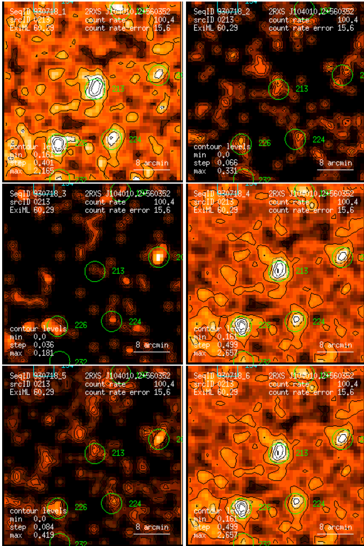
Figure 213: RASS 930718: detection 0213: band rate images, Gaussian filter: (1) PSPC channels 11 – 41, (2) 52 – 90, (3) 91 – 201, (4) 11 – 235, (5) 52 – 201, (6) 11 – 201. Broad band rates in counts/ks. Band rate contour levels in counts/ks/arcmin 2 .
