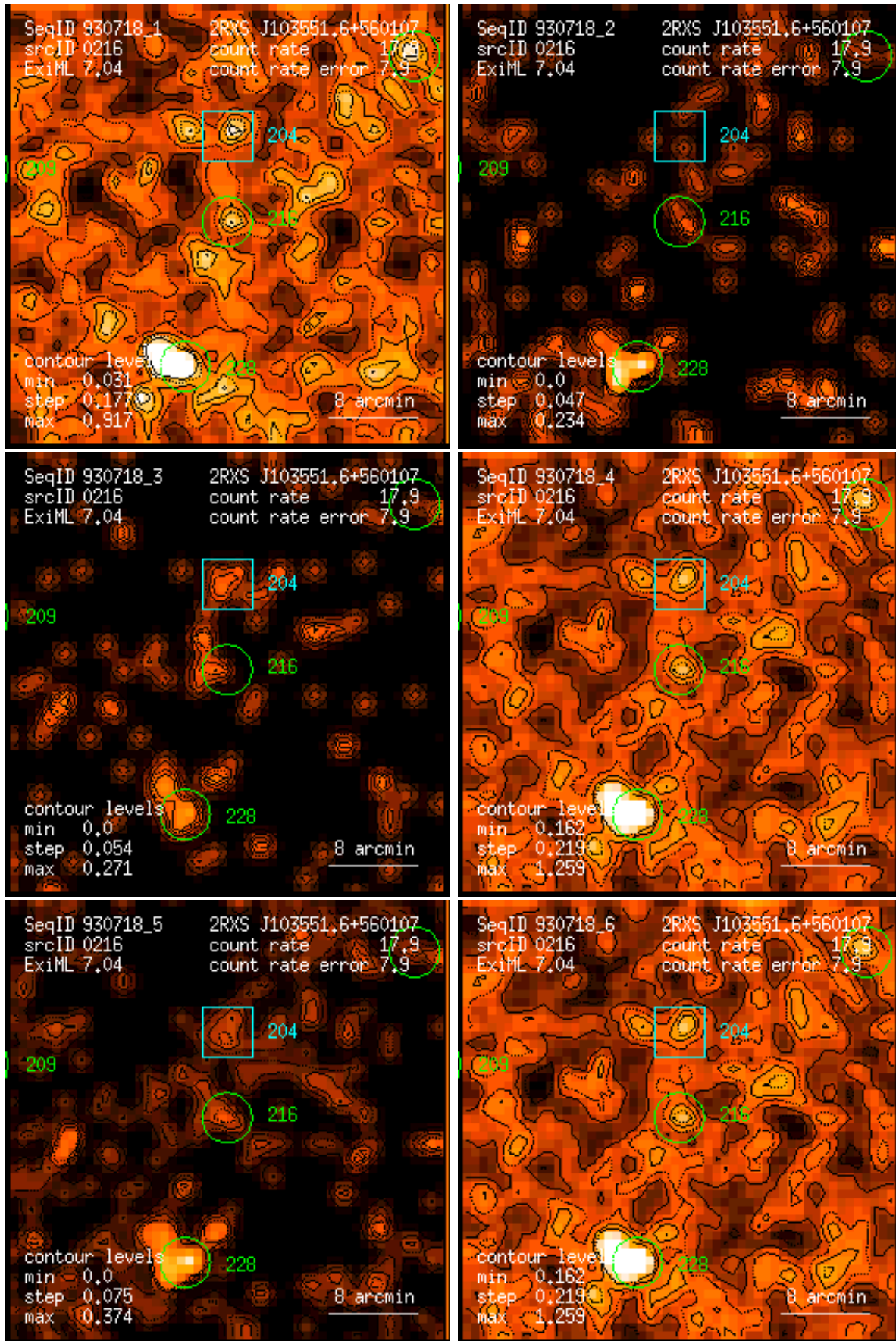
Figure 216: RASS 930718: detection 0216: band rate images, Gaussian filter: (1) PSPC channels 11 – 41, (2) 52 – 90, (3) 91 – 201, (4) 11 – 235, (5) 52 – 201, (6) 11 – 201. Broad band rates in counts/ks. Band rate contour levels in counts/ks/arcmin 2 .
