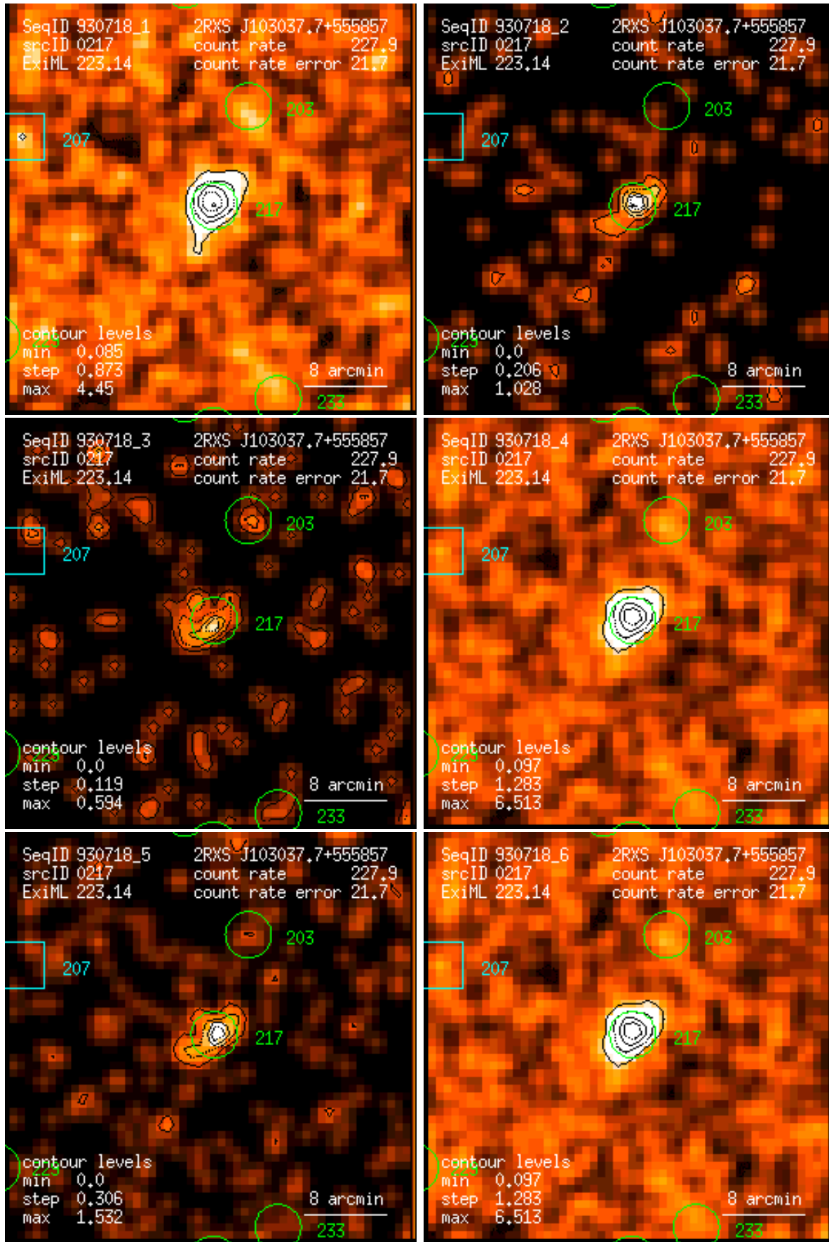
Figure 217: RASS 930718: detection 0217: band rate images, Gaussian filter: (1) PSPC channels 11 – 41, (2) 52 – 90, (3) 91 – 201, (4) 11 – 235, (5) 52 – 201, (6) 11 – 201. Broad band rates in counts/ks. Band rate contour levels in counts/ks/arcmin 2 .
