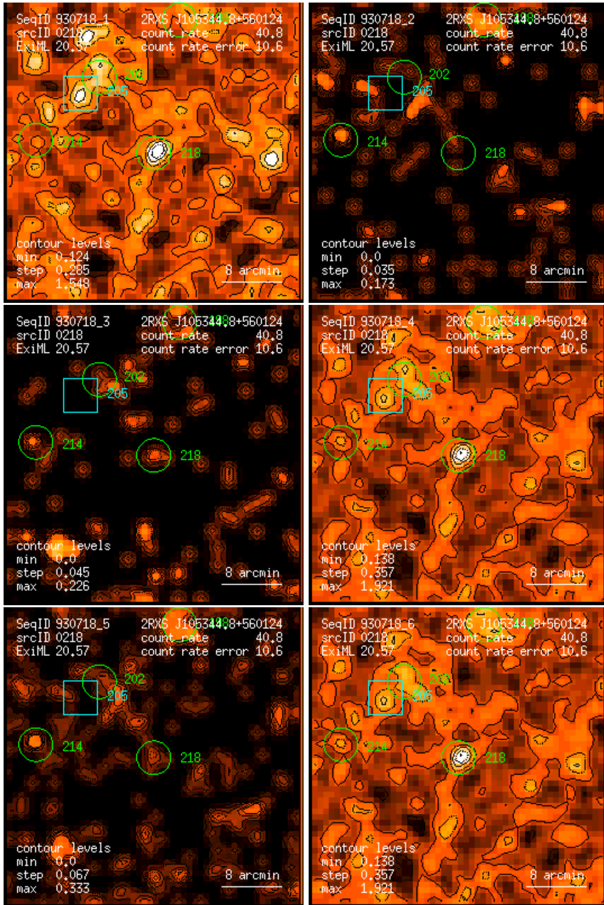
Figure 218: RASS 930718: detection 0218: band rate images, Gaussian filter: (1) PSPC channels 11 – 41, (2) 52 – 90, (3) 91 – 201, (4) 11 – 235, (5) 52 – 201, (6) 11 – 201. Broad band rates in counts/ks. Band rate contour levels in counts/ks/arcmin 2 .
