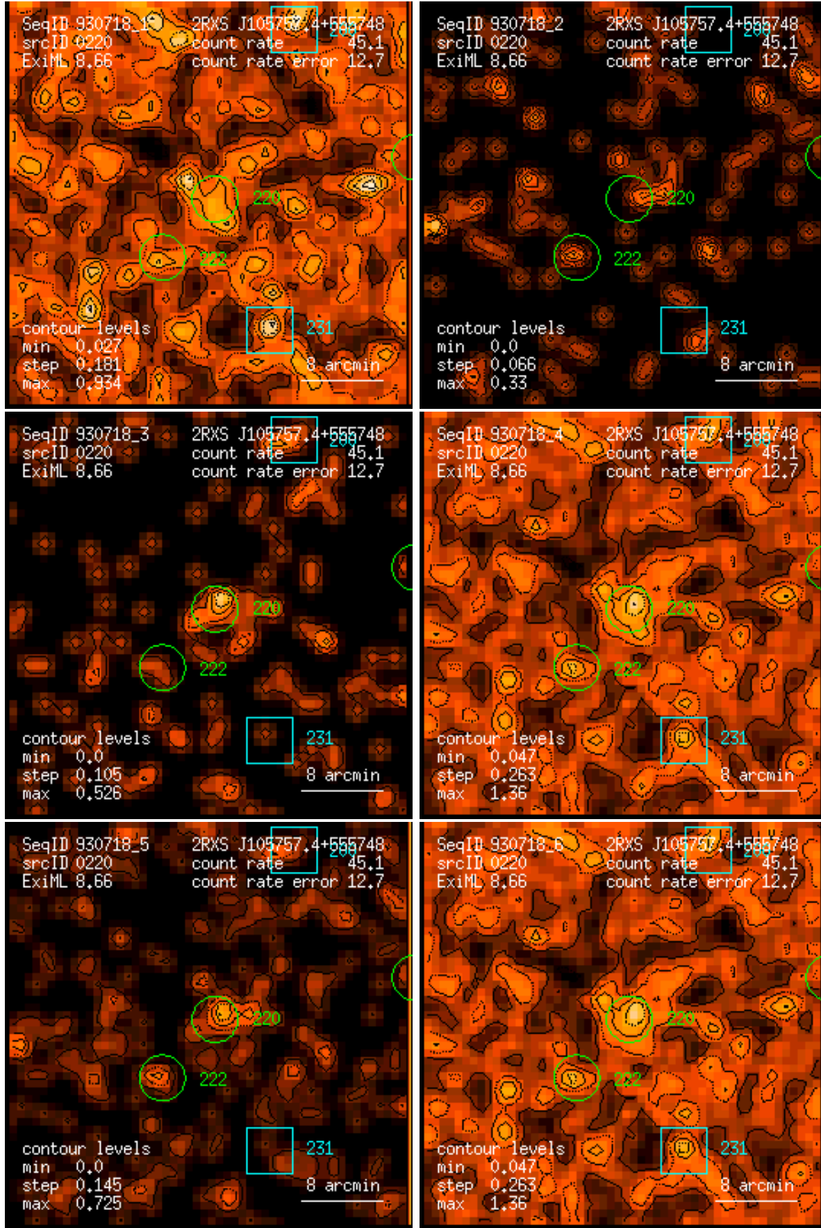
Figure 220: RASS 930718: detection 0220: band rate images, Gaussian filter: (1) PSPC channels 11 – 41, (2) 52 – 90, (3) 91 – 201, (4) 11 – 235, (5) 52 – 201, (6) 11 – 201. Broad band rates in counts/ks. Band rate contour levels in counts/ks/arcmin 2 .
