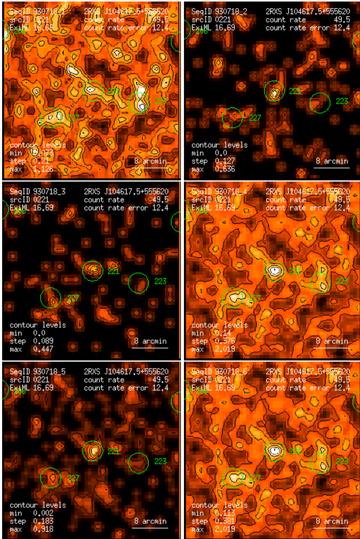
Figure 221: RASS 930718: detection 0221: band rate images, Gaussian filter: (1) PSPC channels 11 – 41, (2) 52 – 90, (3) 91 – 201, (4) 11 – 235, (5) 52 – 201, (6) 11 – 201. Broad band rates in counts/ks. Band rate contour levels in counts/ks/arcmin 2 .
