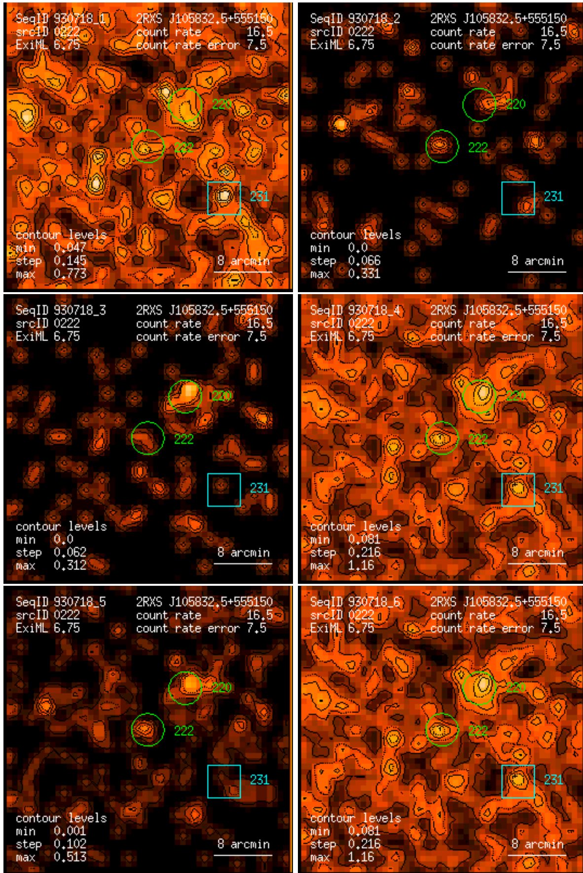
Figure 222: RASS 930718: detection 0222: band rate images, Gaussian filter: (1) PSPC channels 11 – 41, (2) 52 – 90, (3) 91 – 201, (4) 11 – 235, (5) 52 – 201, (6) 11 – 201. Broad band rates in counts/ks. Band rate contour levels in counts/ks/arcmin 2 .
