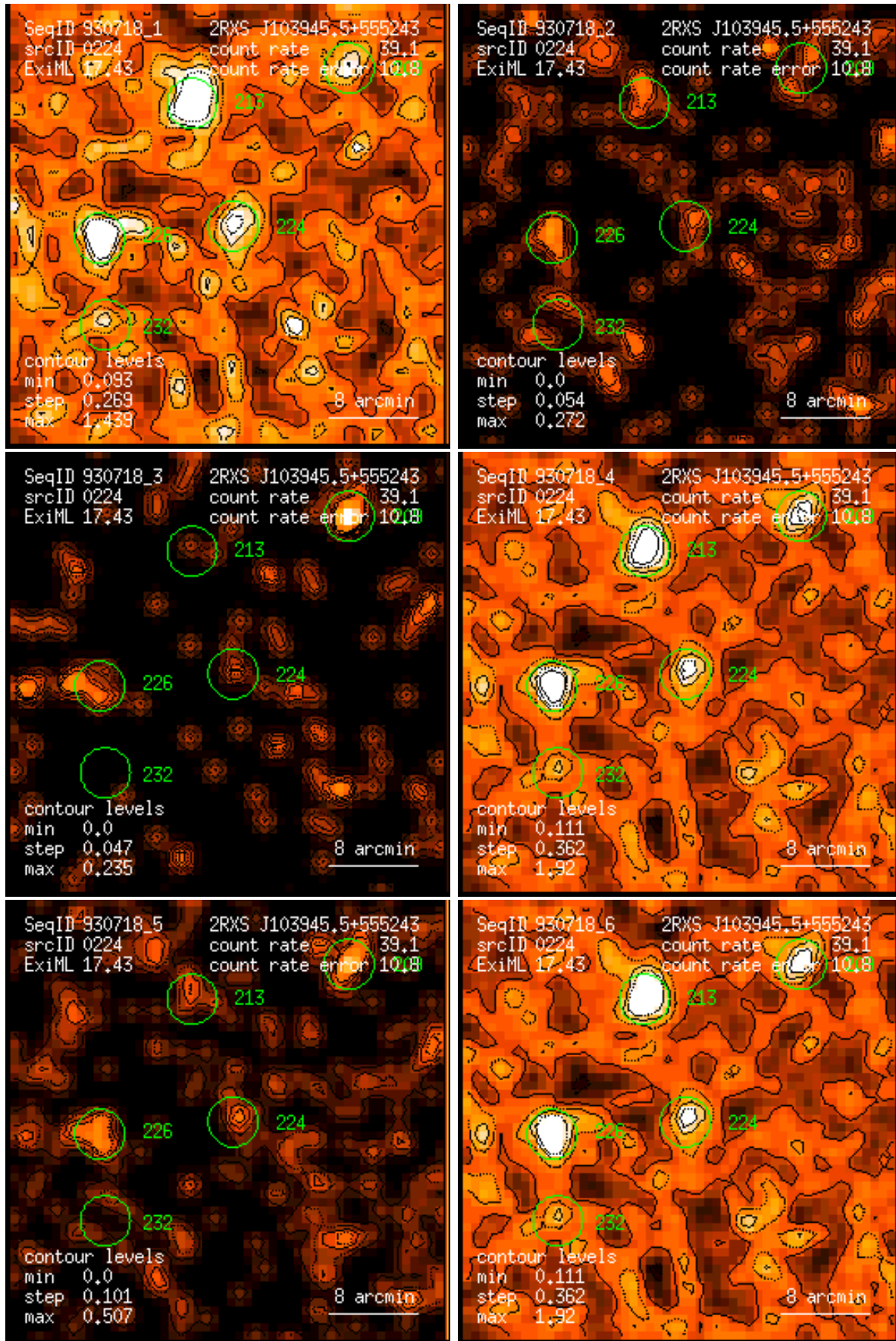
Figure 224: RASS 930718: detection 0224: band rate images, Gaussian filter: (1) PSPC channels 11 – 41, (2) 52 – 90, (3) 91 – 201, (4) 11 – 235, (5) 52 – 201, (6) 11 – 201. Broad band rates in counts/ks. Band rate contour levels in counts/ks/arcmin 2 .
