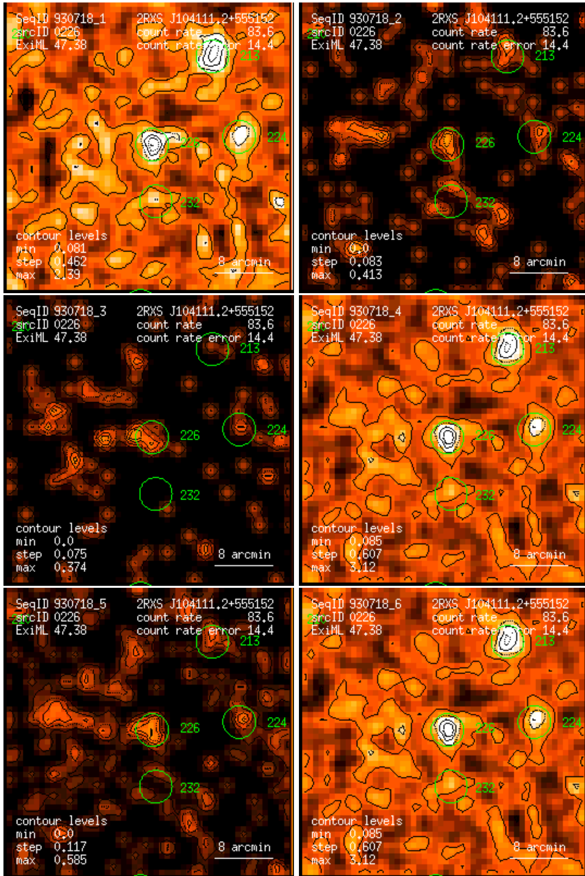
Figure 226: RASS 930718: detection 0226: band rate images, Gaussian filter: (1) PSPC channels 11 – 41, (2) 52 – 90, (3) 91 – 201, (4) 11 – 235, (5) 52 – 201, (6) 11 – 201. Broad band rates in counts/ks. Band rate contour levels in counts/ks/arcmin 2 .
