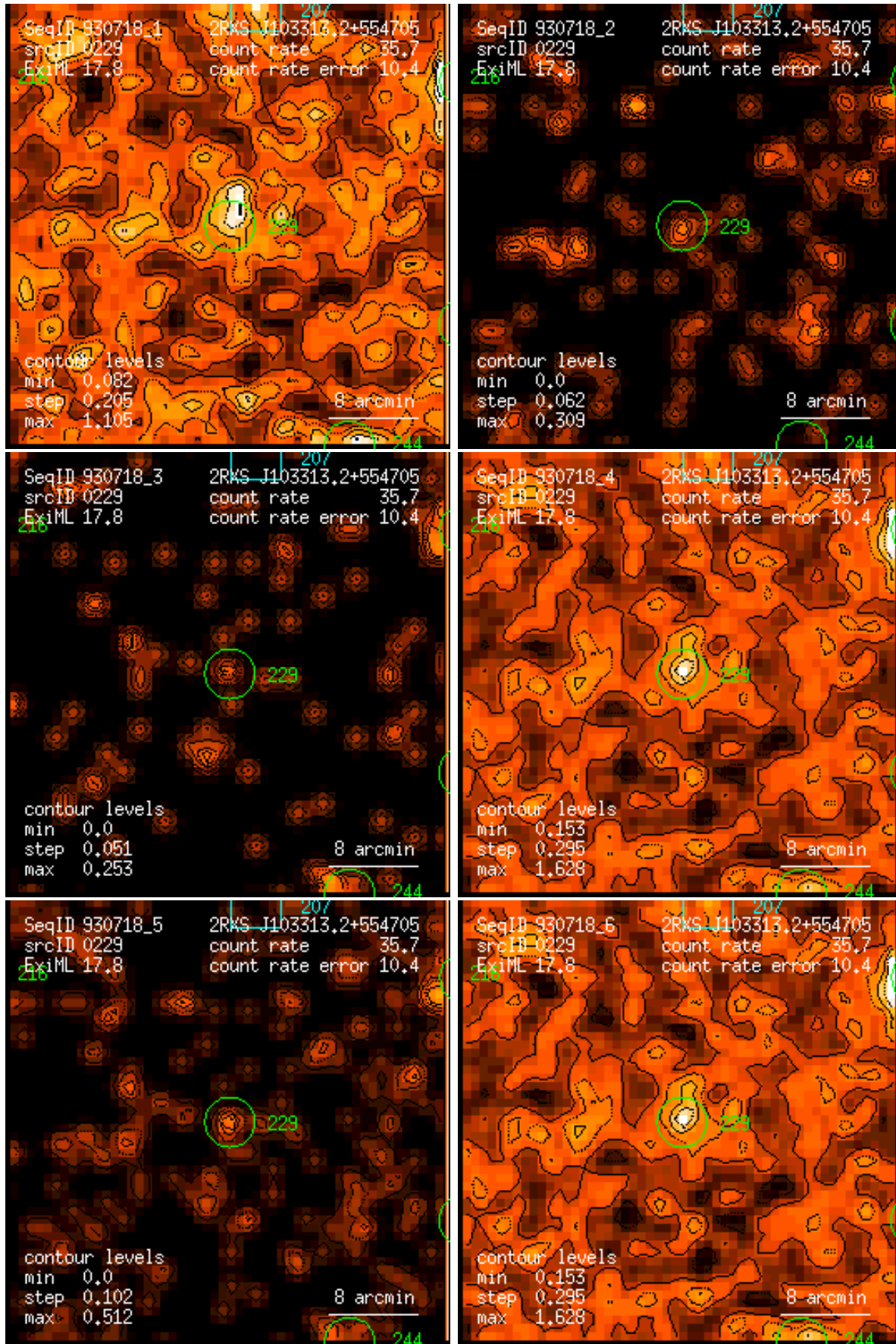
Figure 229: RASS 930718: detection 0229: band rate images, Gaussian filter: (1) PSPC channels 11 – 41, (2) 52 – 90, (3) 91 – 201, (4) 11 – 235, (5) 52 – 201, (6) 11 – 201. Broad band rates in counts/ks. Band rate contour levels in counts/ks/arcmin 2 .
