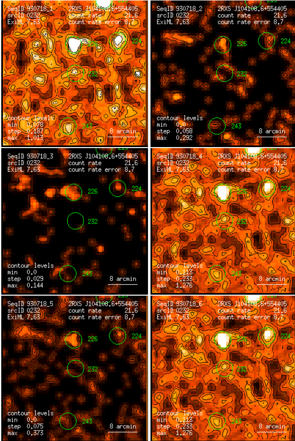
Figure 232: RASS 930718: detection 0232: band rate images, Gaussian filter: (1) PSPC channels 11 – 41, (2) 52 – 90, (3) 91 – 201, (4) 11 – 235, (5) 52 – 201, (6) 11 – 201. Broad band rates in counts/ks. Band rate contour levels in counts/ks/arcmin 2 .
