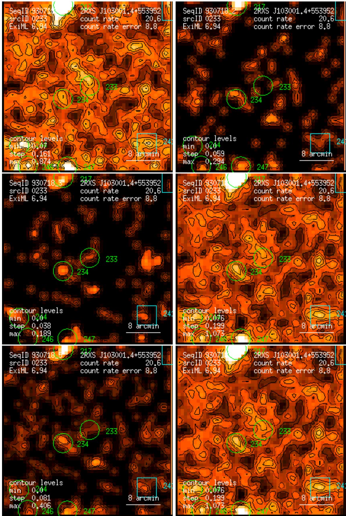
Figure 233: RASS 930718: detection 0233: band rate images, Gaussian filter: (1) PSPC channels 11 – 41, (2) 52 – 90, (3) 91 – 201, (4) 11 – 235, (5) 52 – 201, (6) 11 – 201. Broad band rates in counts/ks. Band rate contour levels in counts/ks/arcmin 2 .
