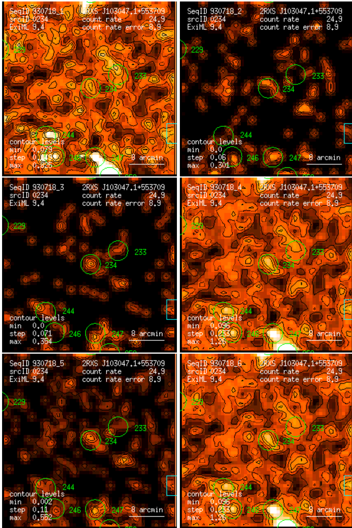
Figure 234: RASS 930718: detection 0234: band rate images, Gaussian filter: (1) PSPC channels 11 – 41, (2) 52 – 90, (3) 91 – 201, (4) 11 – 235, (5) 52 – 201, (6) 11 – 201. Broad band rates in counts/ks. Band rate contour levels in counts/ks/arcmin 2 .
