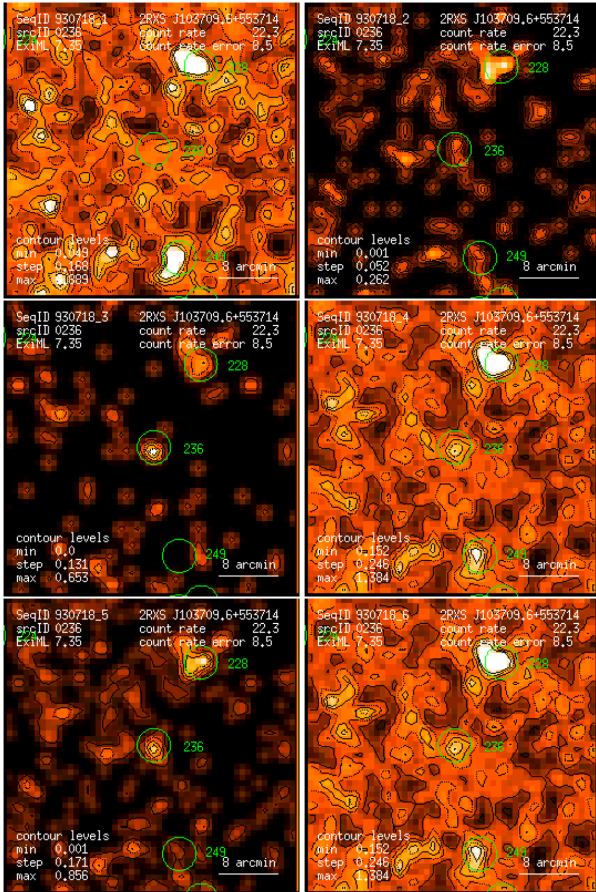
Figure 236: RASS 930718: detection 0236: band rate images, Gaussian filter: (1) PSPC channels 11 – 41, (2) 52 – 90, (3) 91 – 201, (4) 11 – 235, (5) 52 – 201, (6) 11 – 201. Broad band rates in counts/ks. Band rate contour levels in counts/ks/arcmin 2 .
