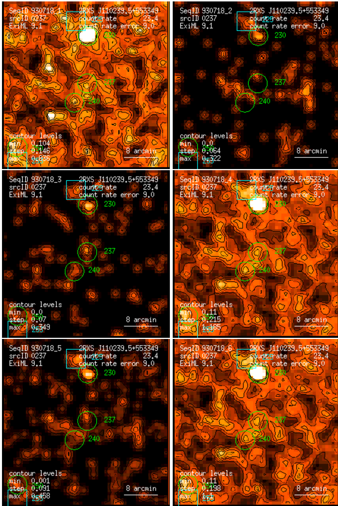
Figure 237: RASS 930718: detection 0237: band rate images, Gaussian filter: (1) PSPC channels 11 – 41, (2) 52 – 90, (3) 91 – 201, (4) 11 – 235, (5) 52 – 201, (6) 11 – 201. Broad band rates in counts/ks. Band rate contour levels in counts/ks/arcmin 2 .
