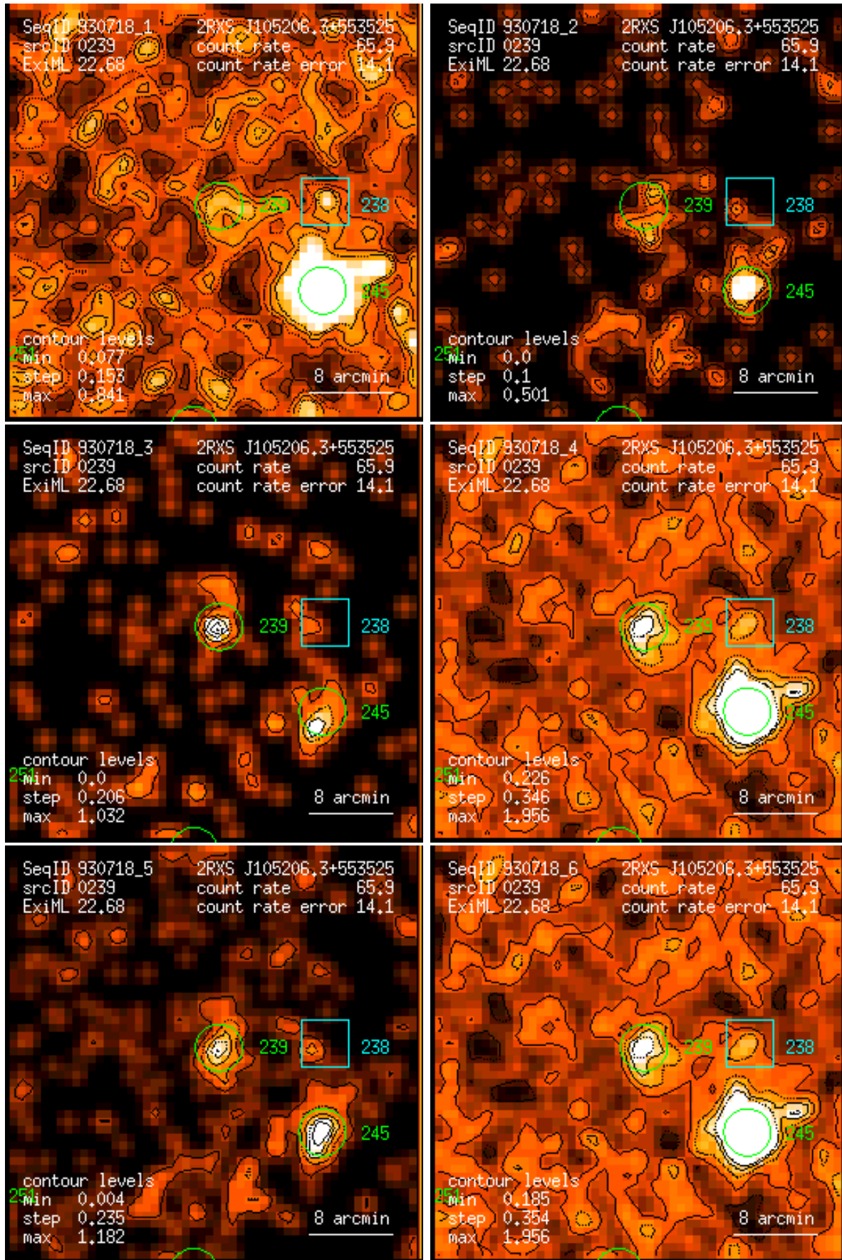
Figure 239: RASS 930718: detection 0239: band rate images, Gaussian filter: (1) PSPC channels 11 – 41, (2) 52 – 90, (3) 91 – 201, (4) 11 – 235, (5) 52 – 201, (6) 11 – 201. Broad band rates in counts/ks. Band rate contour levels in counts/ks/arcmin 2 .
