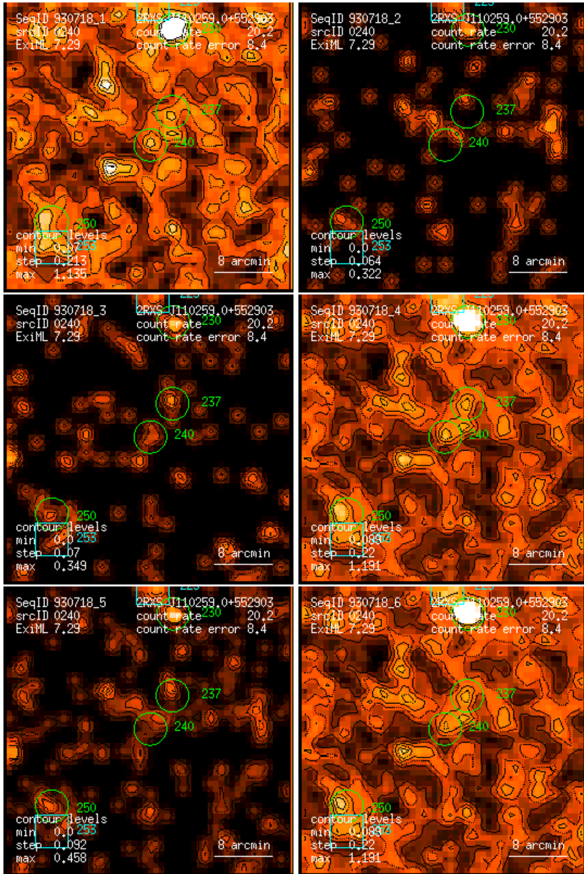
Figure 240: RASS 930718: detection 0240: band rate images, Gaussian filter: (1) PSPC channels 11 – 41, (2) 52 – 90, (3) 91 – 201, (4) 11 – 235, (5) 52 – 201, (6) 11 – 201. Broad band rates in counts/ks. Band rate contour levels in counts/ks/arcmin 2 .
