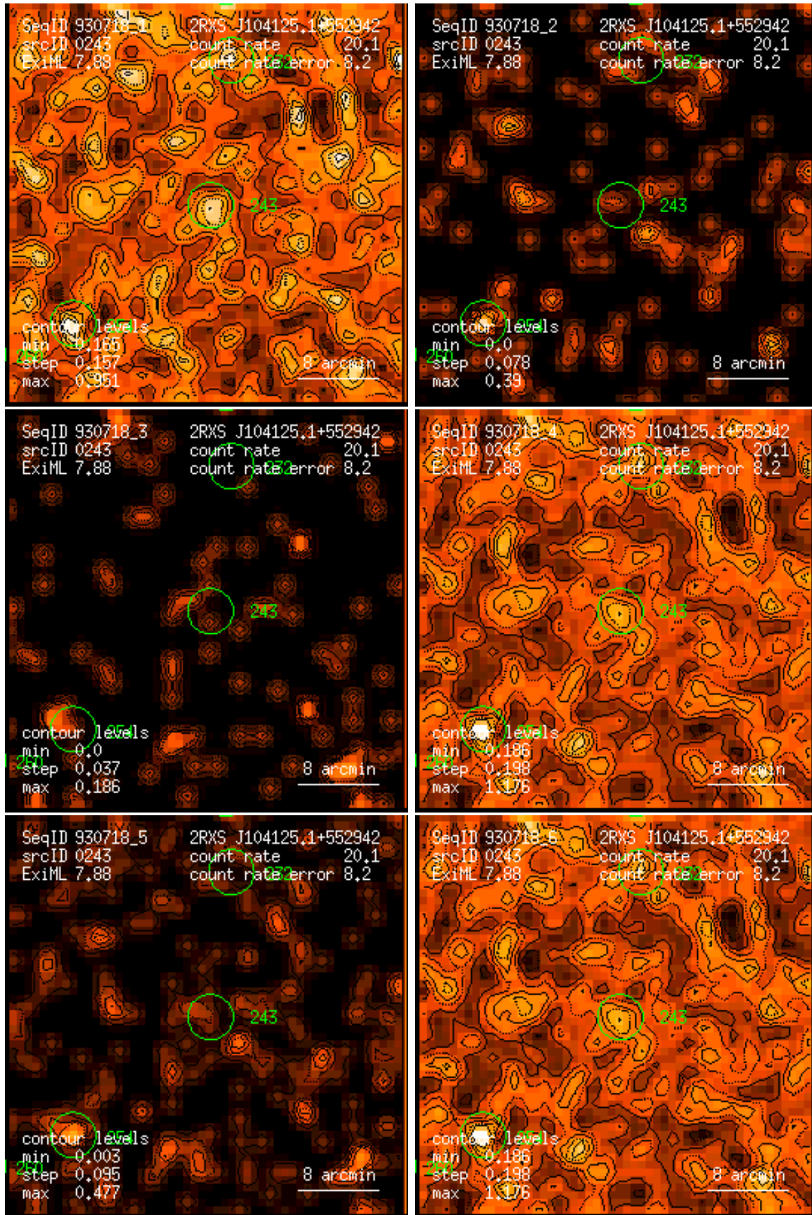
Figure 243: RASS 930718: detection 0243: band rate images, Gaussian filter: (1) PSPC channels 11 – 41, (2) 52 – 90, (3) 91 – 201, (4) 11 – 235, (5) 52 – 201, (6) 11 – 201. Broad band rates in counts/ks. Band rate contour levels in counts/ks/arcmin 2 .
